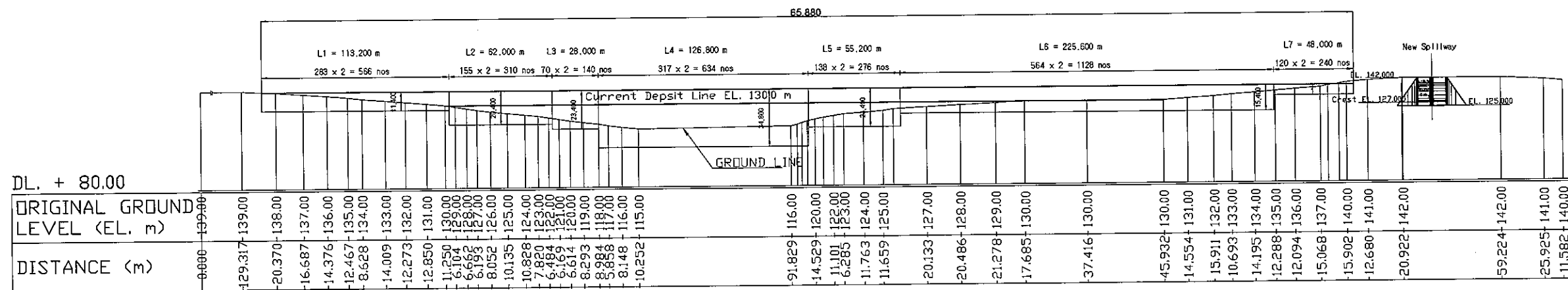
LONGITUDINAL PROFILE OF CLOSURE DIKE Scale : 1 : 2500
