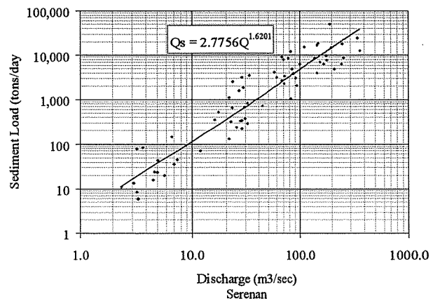
Figure 1.2.12 Sediment Discharge Rating Curves in Upper Solo River Basin
