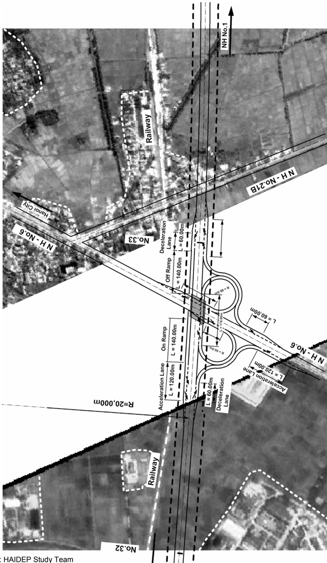
Figure 3.4.6 Intersection Plan for NH6 and RR4
