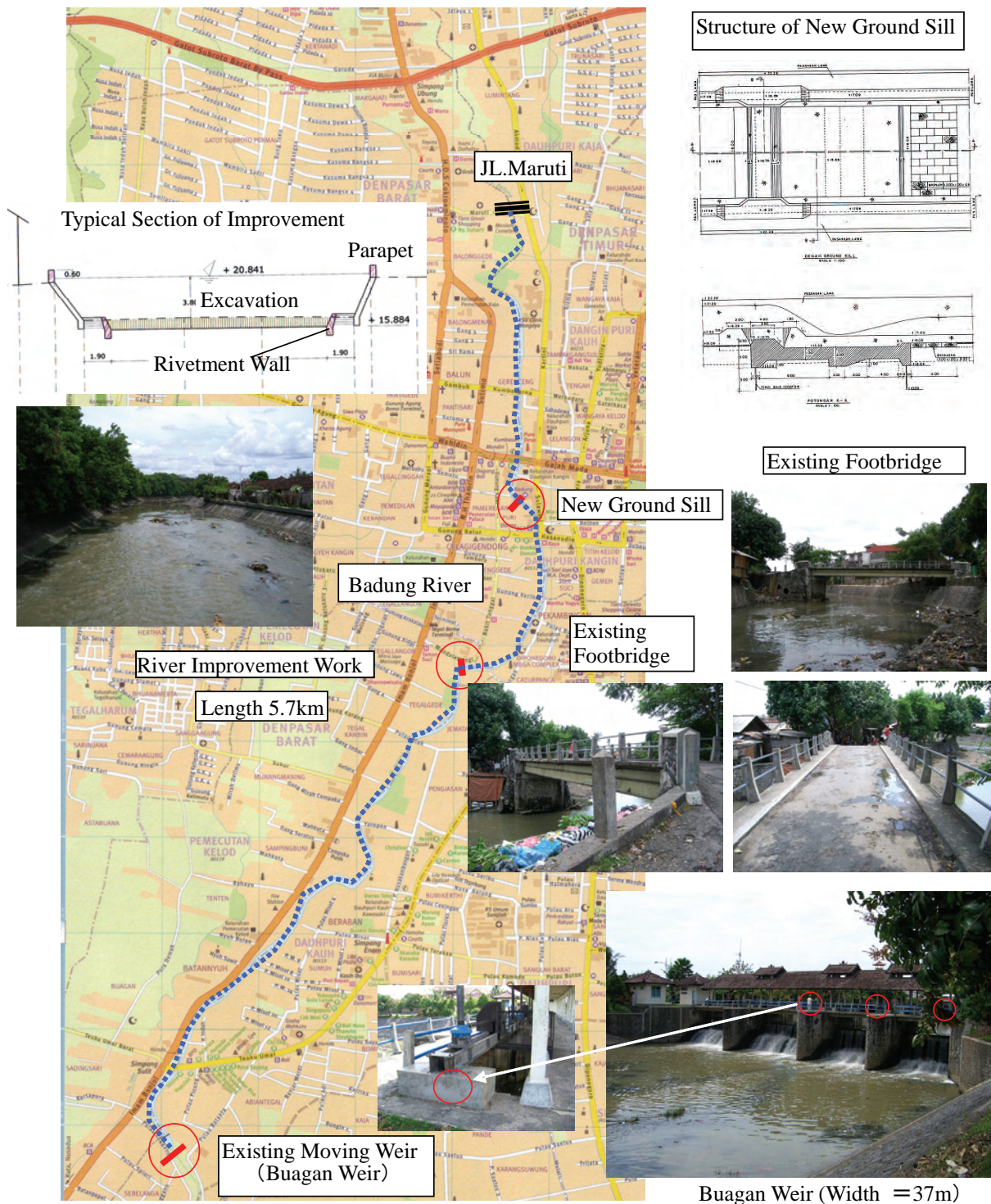
Figure-5.23 General Plan Flood Prevention Project for Badung River
