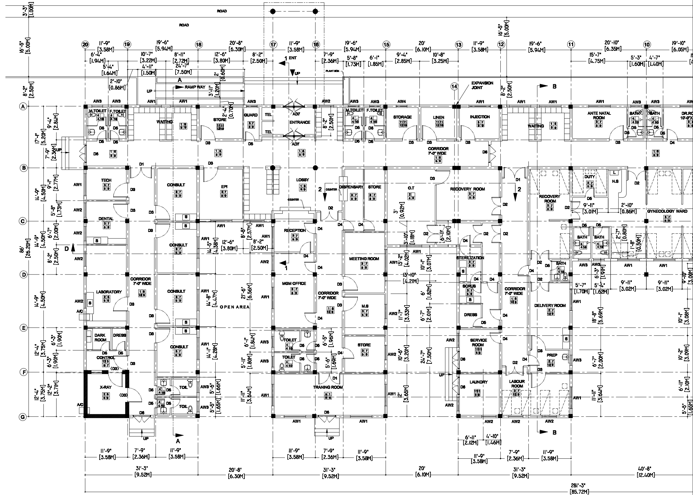
GENERAL FLOOR PLAN-1 S=1:200
