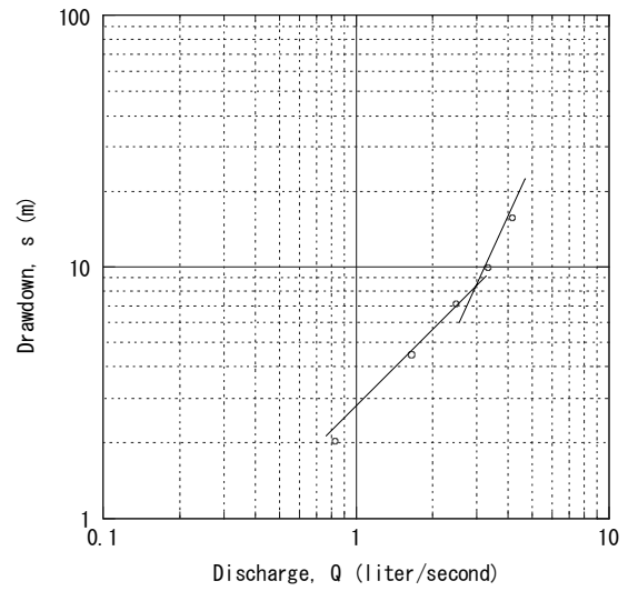
Dekemhare Enda Asale2 (Existing) Step-Drawdown Test
