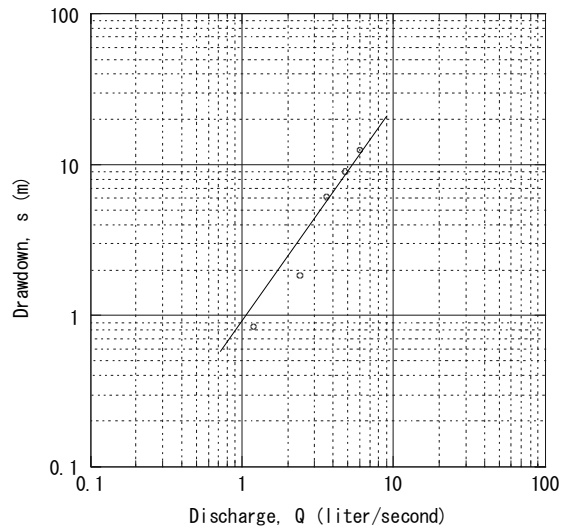
Adi Keyih No. 17 Step-Drawdown Test
