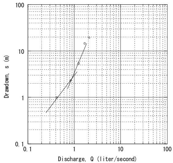
Debarwa BH12 (Existing) Step-Drawdown Test in Dry Season
