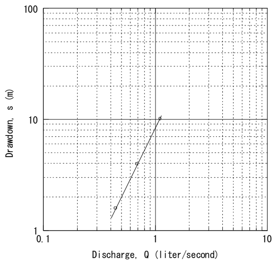
May-dima PW-1 (Existing) Step-Drawdown Test
