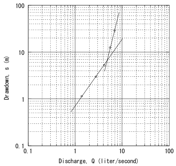
Adi Keyih No. 19 Step-Drawdown Test
