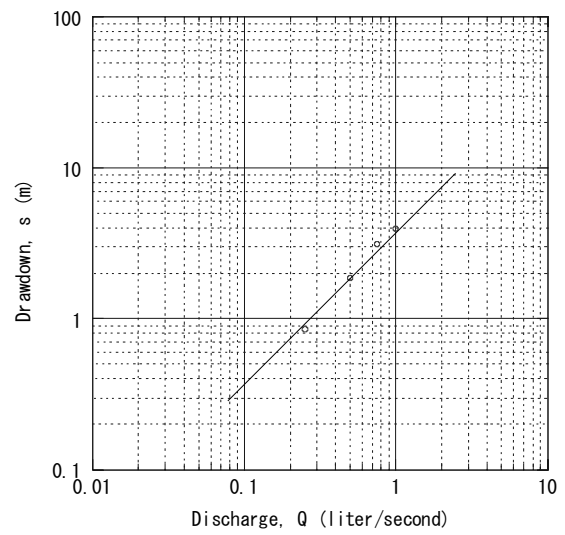
May-dima No.7 Step-Drawdown Test
