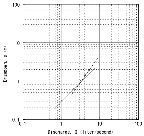
Adi Keyih No. 18 Step-Drawdown Test in Dry Season
