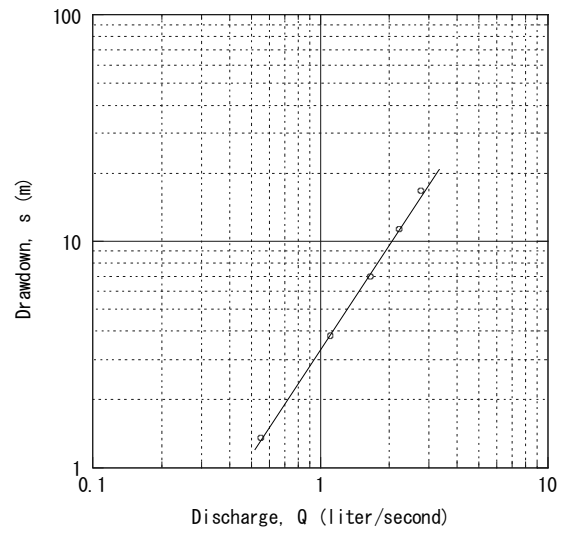
Debarwa No. 10 Step-Drawdown Test
