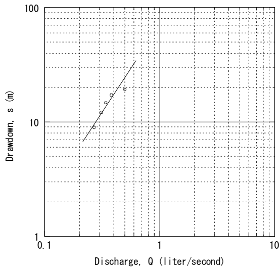
Debarwa No. 7 Step-Drawdown Test
