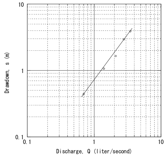
Adi Keyih BH3 (Existing) Step-Drawdown Test
