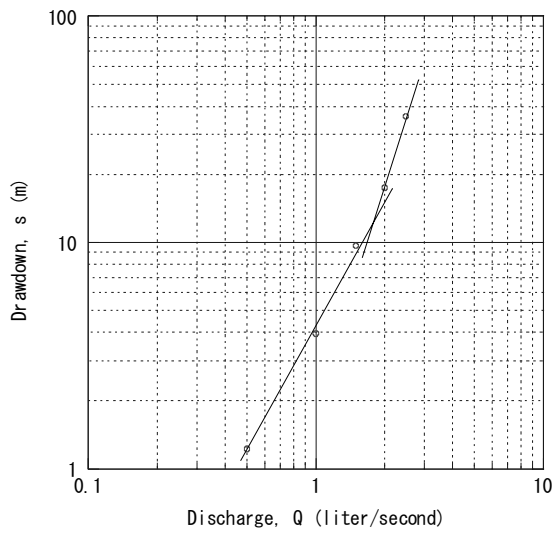
Debarwa No. 11-1 Step-Drawdown Test
