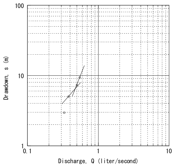
May-dima No.1 Step-Drawdown Test
