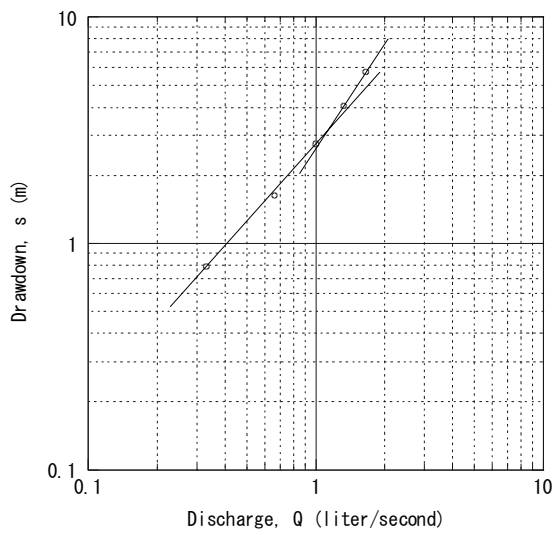
Dekemhare No. 2 Step-Drawdown Test
