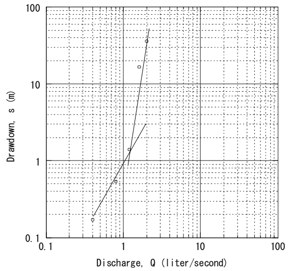
Adi Keyih No. 13 Step-Drawdown Test
