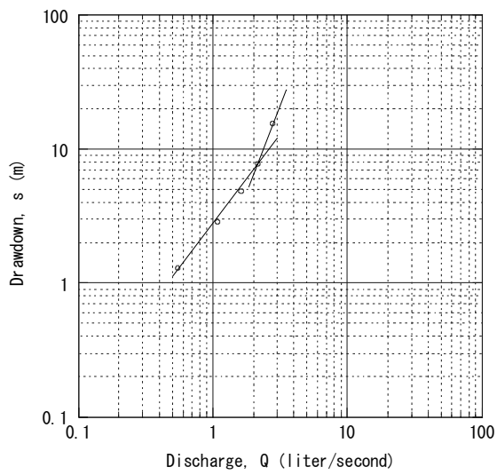
Adi Keyih No. 14 Step-Drawdown Test
