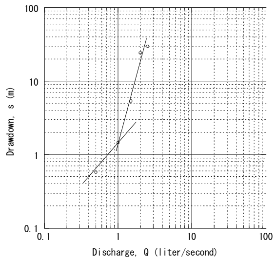
May-dima Existing PW-2 Step-Drawdown Test in Dry Season
