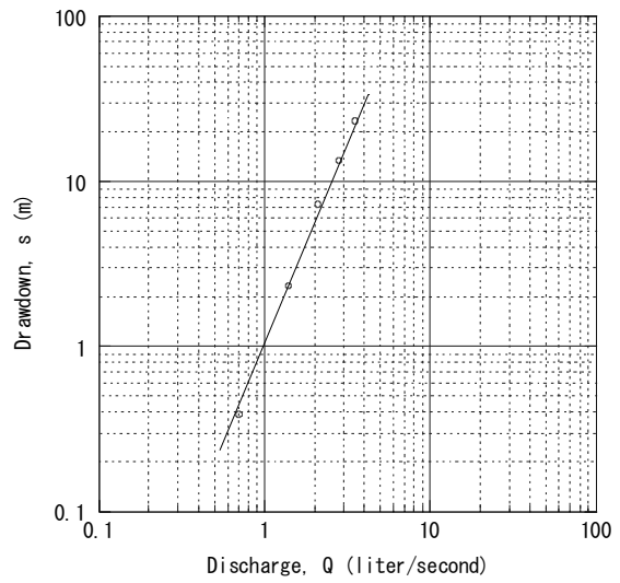
Adi Keyih AD12 (Existing) Step-Drawdown Test
