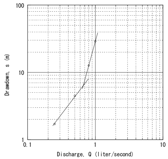
Adi Keyih No.7 Step-Drawdown Test
