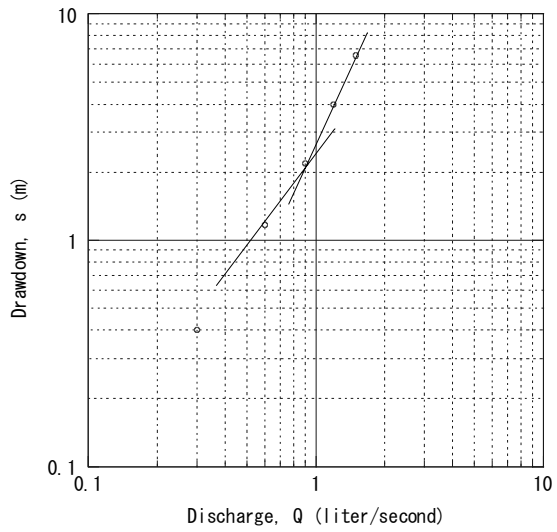
Adi Keyih No. 9 Step-Drawdown Test
