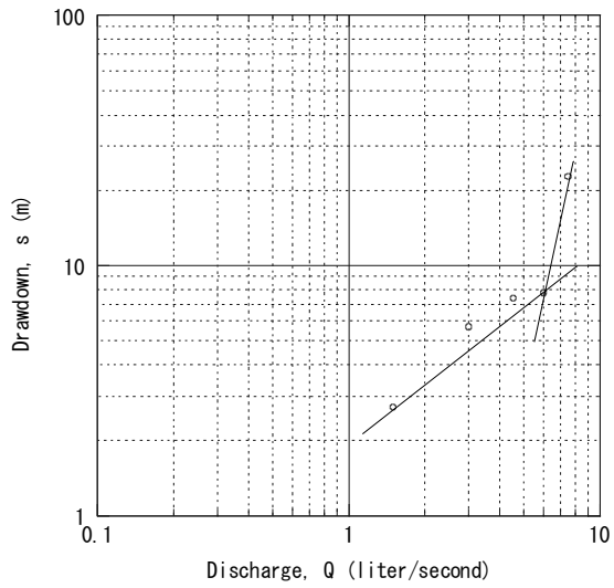
Dekemhare No. 4 Step-Drawdown Test
