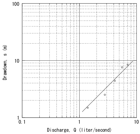
Adi Keyih No. 16 Step-Drawdown Test
