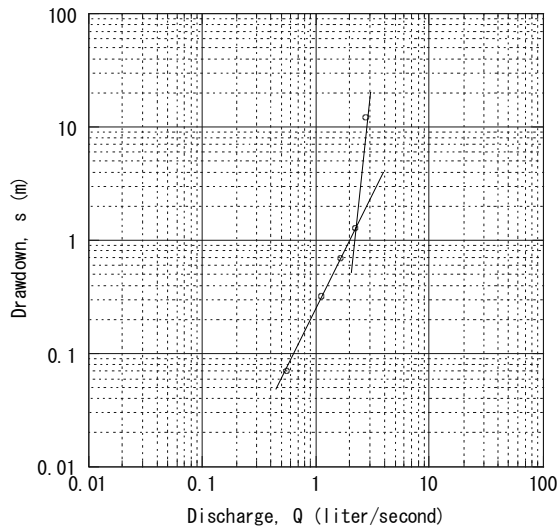
Debarwa DEB-1 (Existing) Step-Drawdown Test
