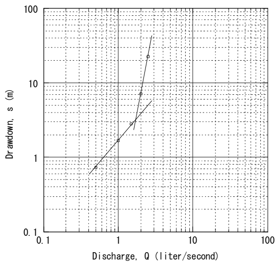
Adi Keyih No.6 Step-Drawdown Test
