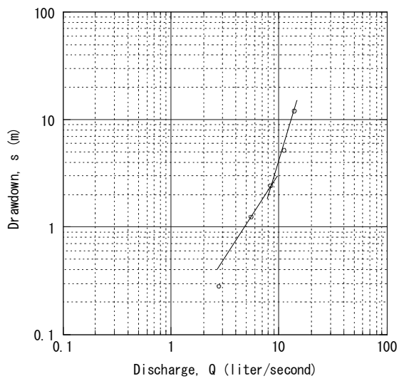
Adi Keyih No. 18 Step-Drawdown Test
