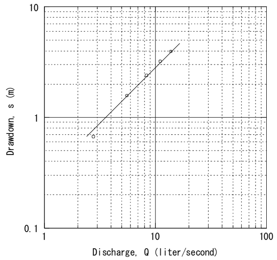
Dekemhare No. 5 Step-Drawdown Test
