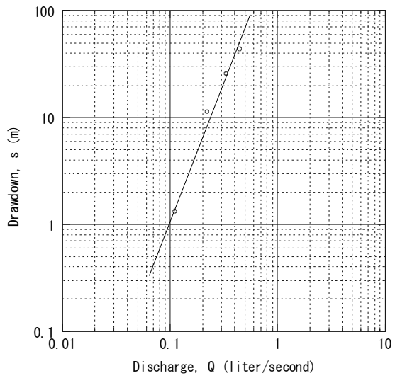
May-dima No. 7 Step-Drawdown Test in Dry Season
