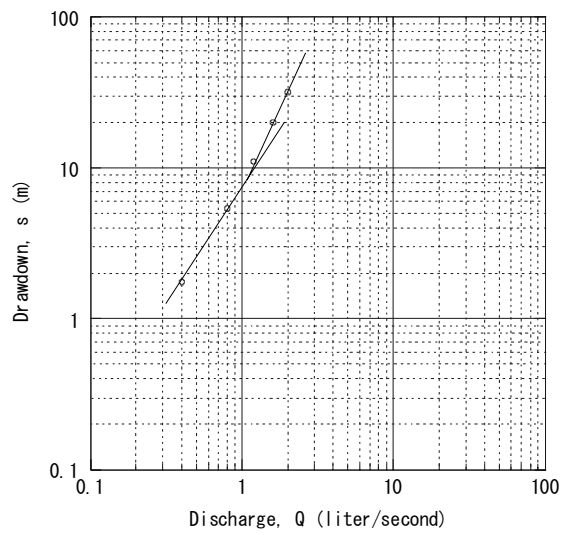
Adi Keyih No. 15 Step-Drawdown Test
