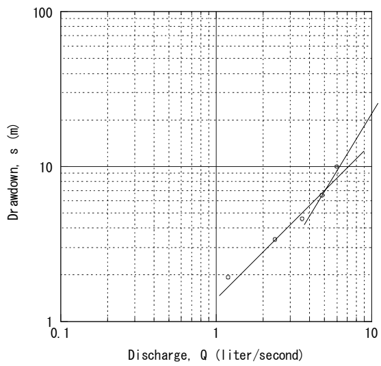
Adi Keyih No. 16 Step-Drawdown Test in Dry Season
