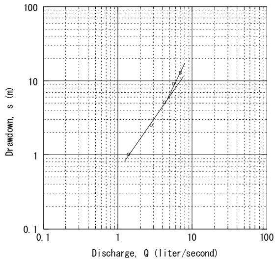
Dekemhare DEK-2 (Existing) Step-Drawdown Test
