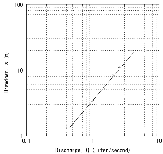
Debarwa 11-2 Step-Drawdown Test in Dry Season
