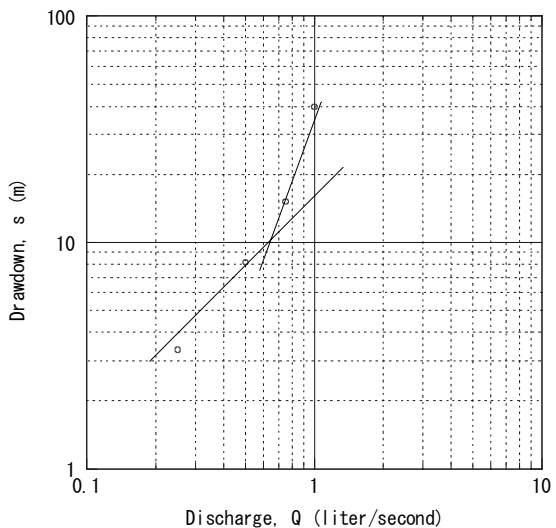
May-dima No.1 Step-Drawdown Test in Dry Season
