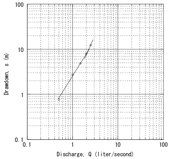
Dekemhare No. 1 Step-Drawdown Test
