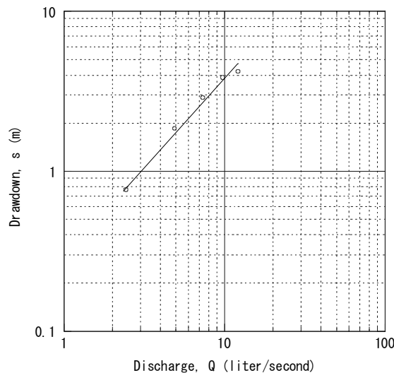
Dekemhare No. 5 Step-Drawdown Test in Dry Season
