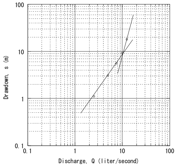
Adi Keyih No. 20 Step-Drawdown Test
