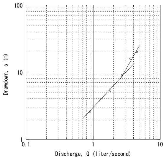
Dekemhare BH14 (Existing) Step-Drawdown Test
