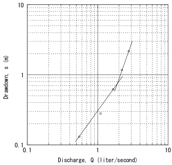
Adi Keyih BH7 (Existing) Step-Drawdown Test
