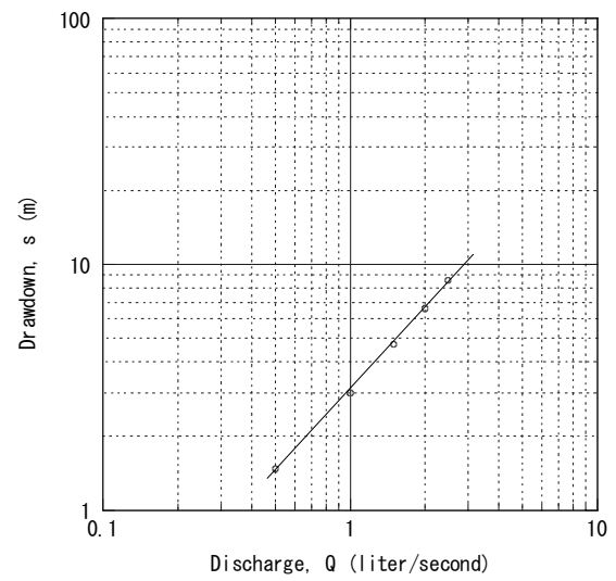
Dekemhare No. 3 Step-Drawdown Test
