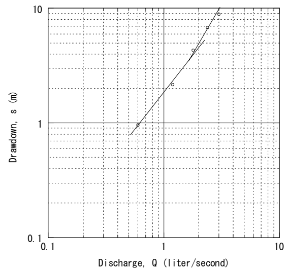
Dekemhare BH19 (Existing) Step-Drawdown Test
