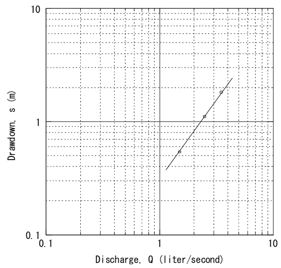
Adi Keyih Hawatsu (Existing) Step-Drawdown Test
