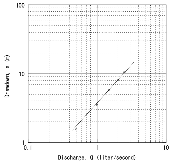
Debarwa No. 11-2 Step-Drawdown Test
