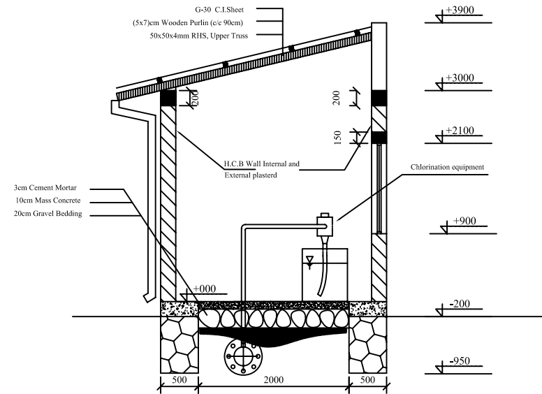
SECTION C-C
