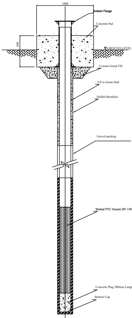
DRILLED BOREHOLE AND CASING
