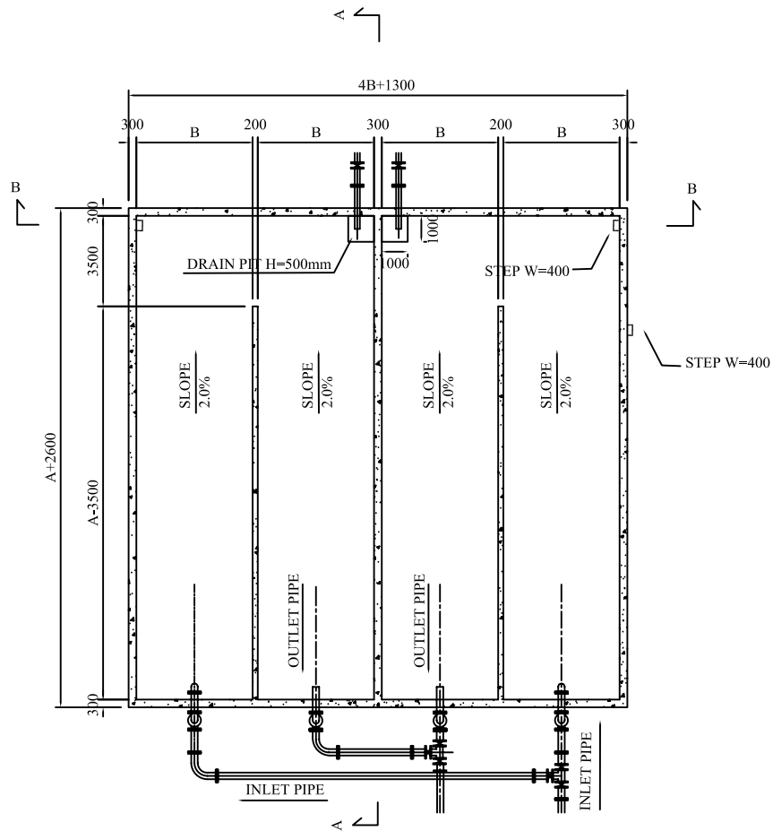
RESERVOIR PLAN
