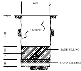
STANDARD CROSS SECTION D 50 ~ 150mm
