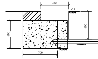
TYPICAL SECTION
