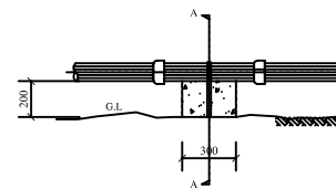
THRUST BLOCK
