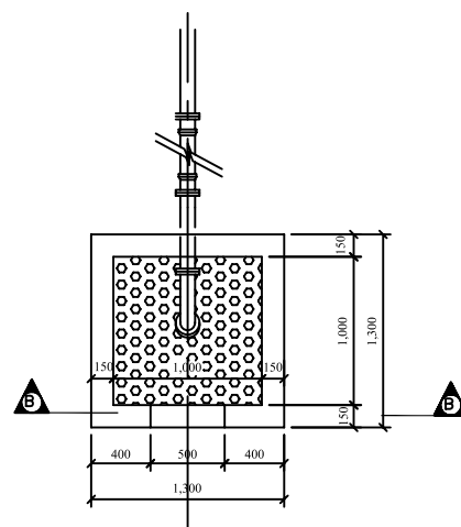
OUTFALL PLAN
