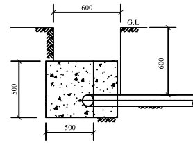
TYPICAL SECTION
