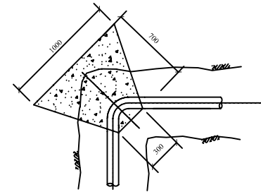
TRUST BLOCK PIPE MORE THAN D200
