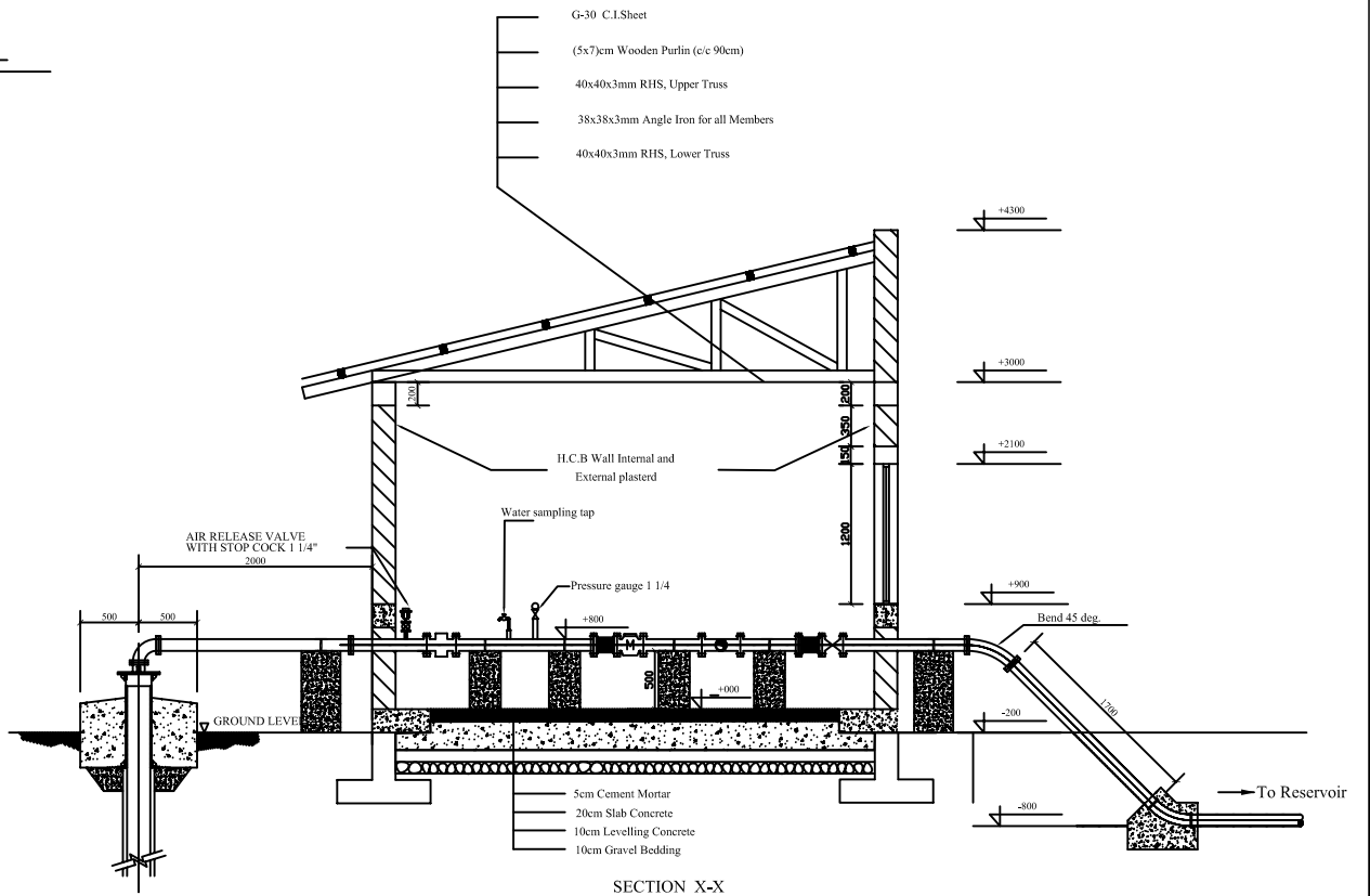
SECTION X-X
