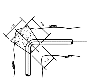
TRUST BLOCK PIPE LESS THAN D150
