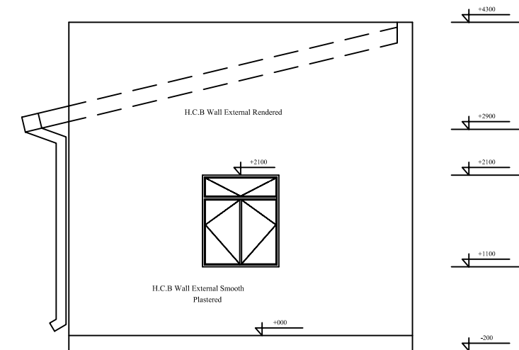
SIDE ELEVATION
