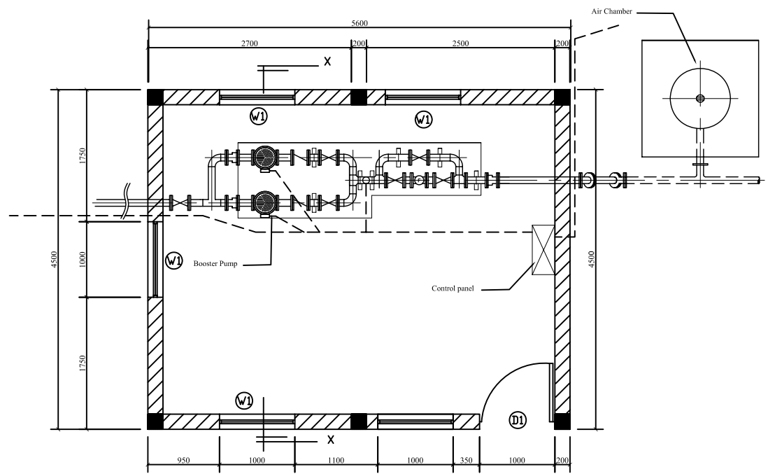
FLOOR PLAN
