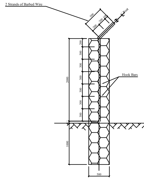
SIDE VIEW OF GATE POST
