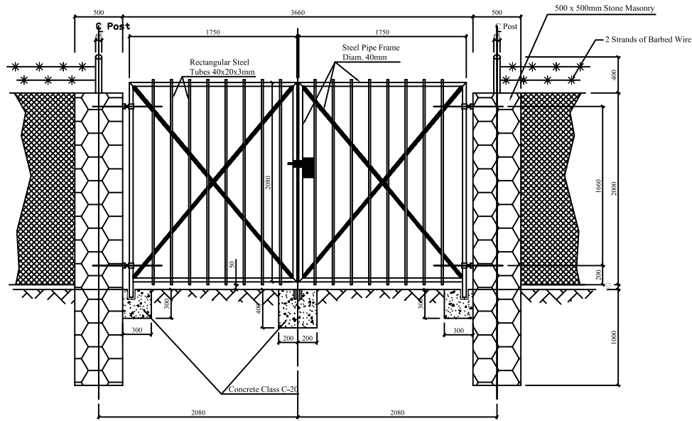
REAR ELEVATION OF GATE
