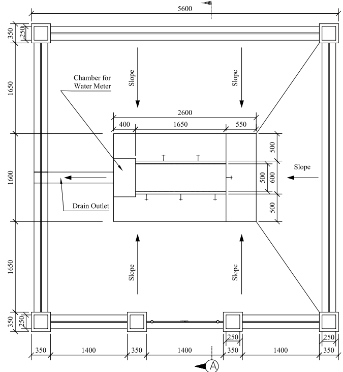
PLAN OF PUBLIC FOUNTAIN
