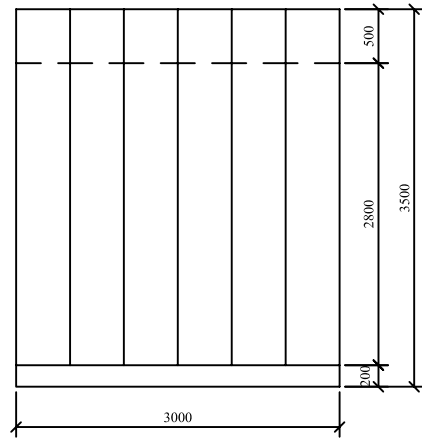
ROOF PLAN
