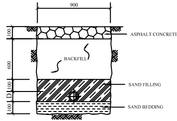
ASPHALT ROAD REPAIRING SECTION D 200 mm ~
