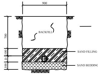
STANDARD CROSS SECTION D 200 mm ~
