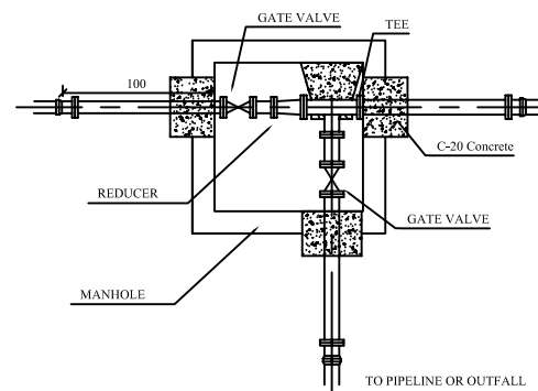
GATE VALVE & FITTINGS PLAN
