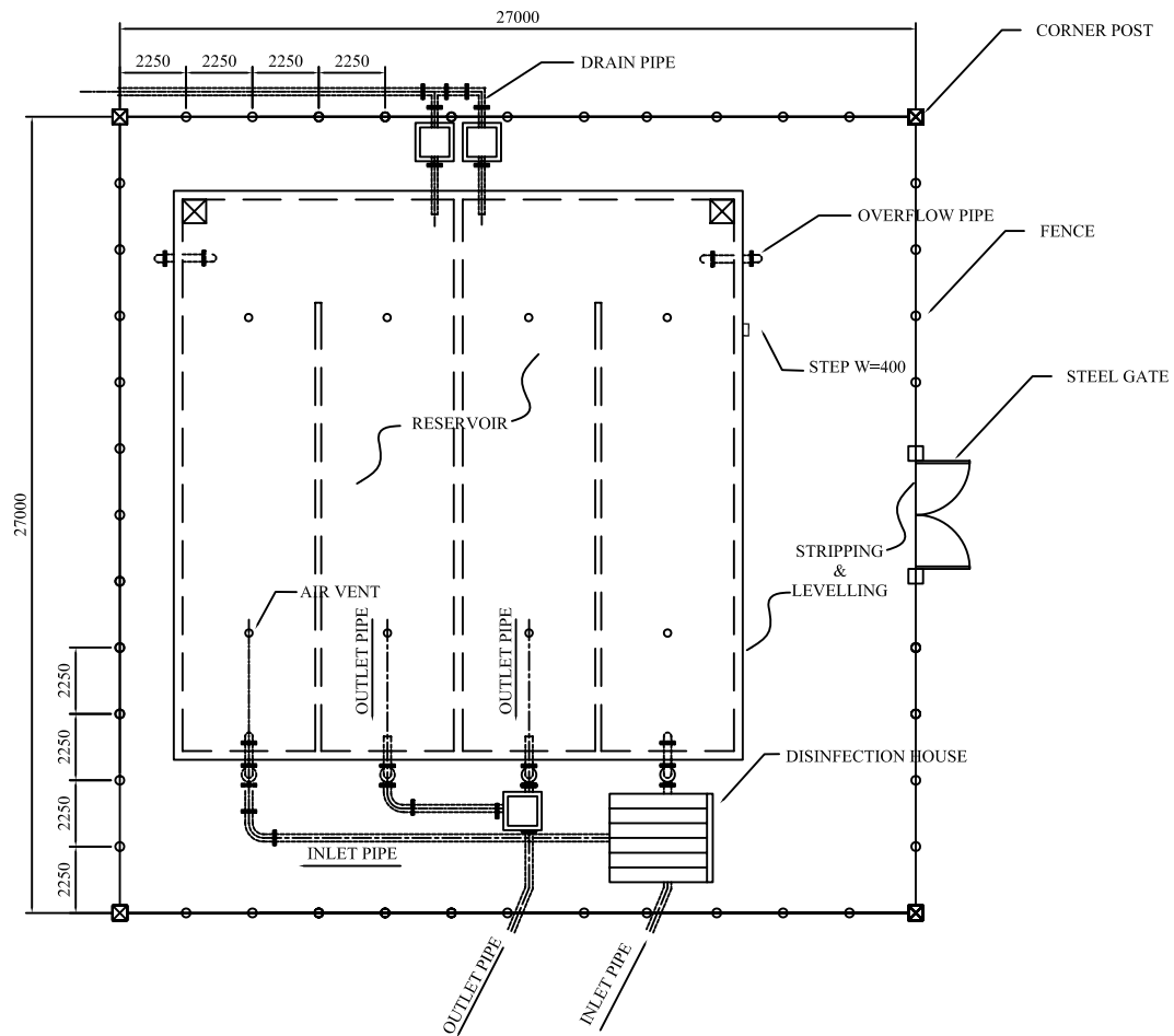
LAYOUT PLAN
