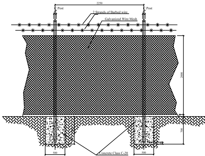
ELEVATION VIEW OF FENCE
