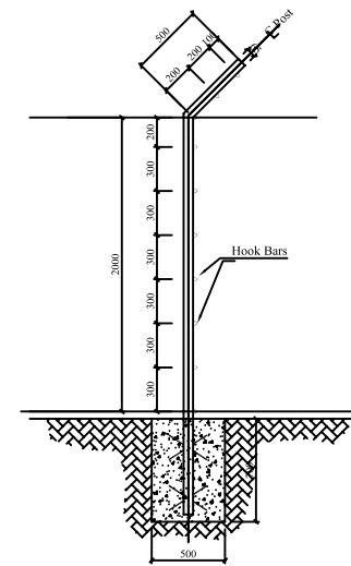
SIDE VIEW OF FENCE
