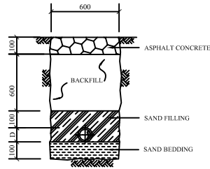
ASPHALT ROAD REPAIRING SECTION D 50 ~ 150mm
