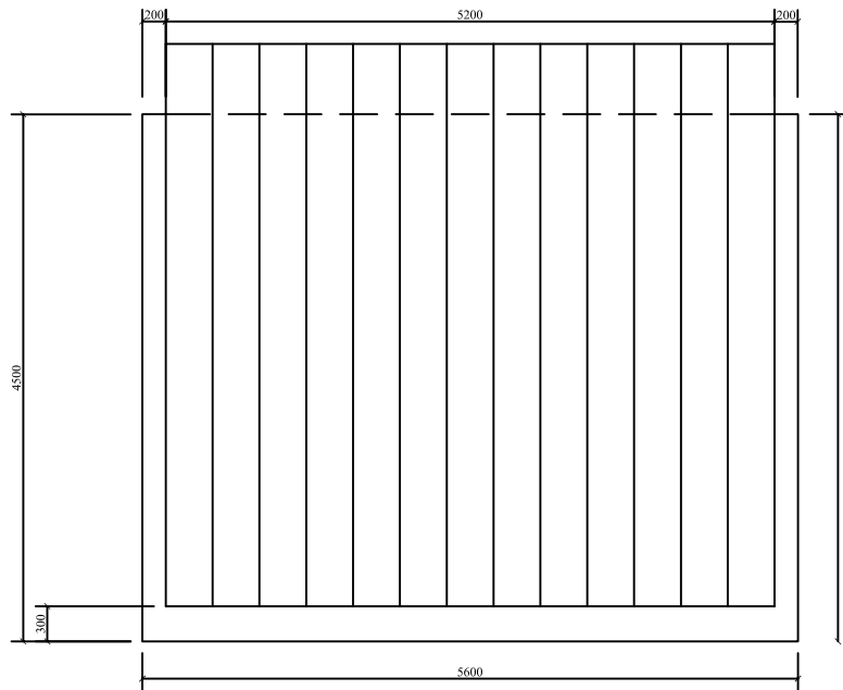
ROOF PLAN
