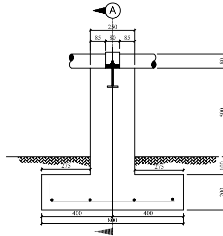
PIPE SUPPORT
