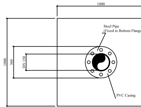
BOREHOLE PLAN VIEW
