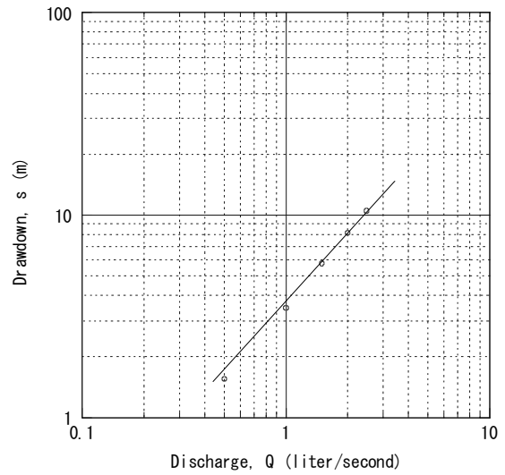
Debarwa No. 11-2 Step-Drawdown Test
