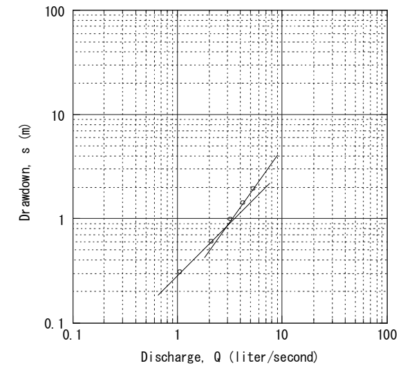
Adi Keyih No. 18 Step-Drawdown Test in Dry Season
