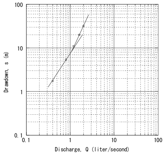
Adi Keyih No. 15 Step-Drawdown Test
