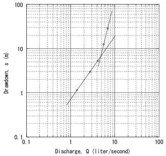
Adi Keyih No. 19 Step-Drawdown Test
