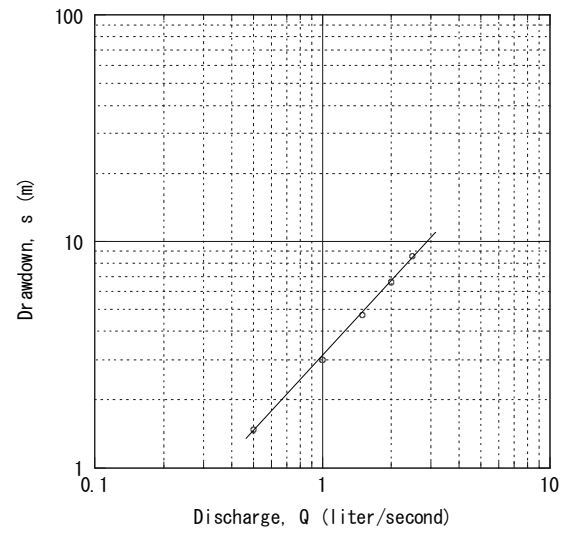
Dekemhare No. 3 Step-Drawdown Test
