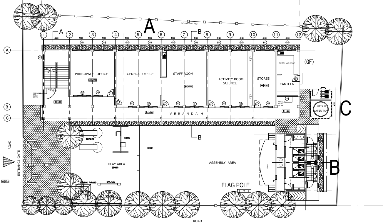
LAYOUT PLAN
