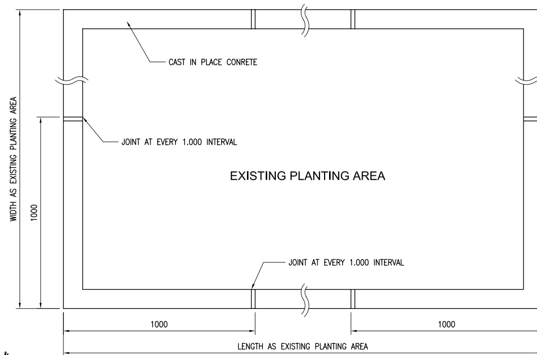
PLAN SCALE 1:20
