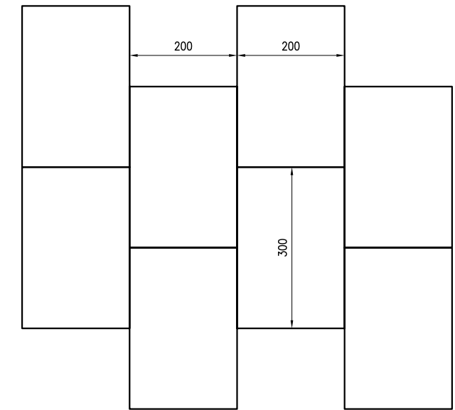
PLAN SCALE 1:10
