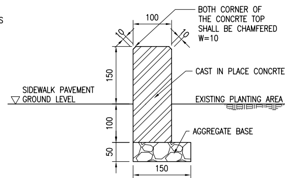
PLANTING AREA CONCRETE EDGE TRIM SCALE 1:10
