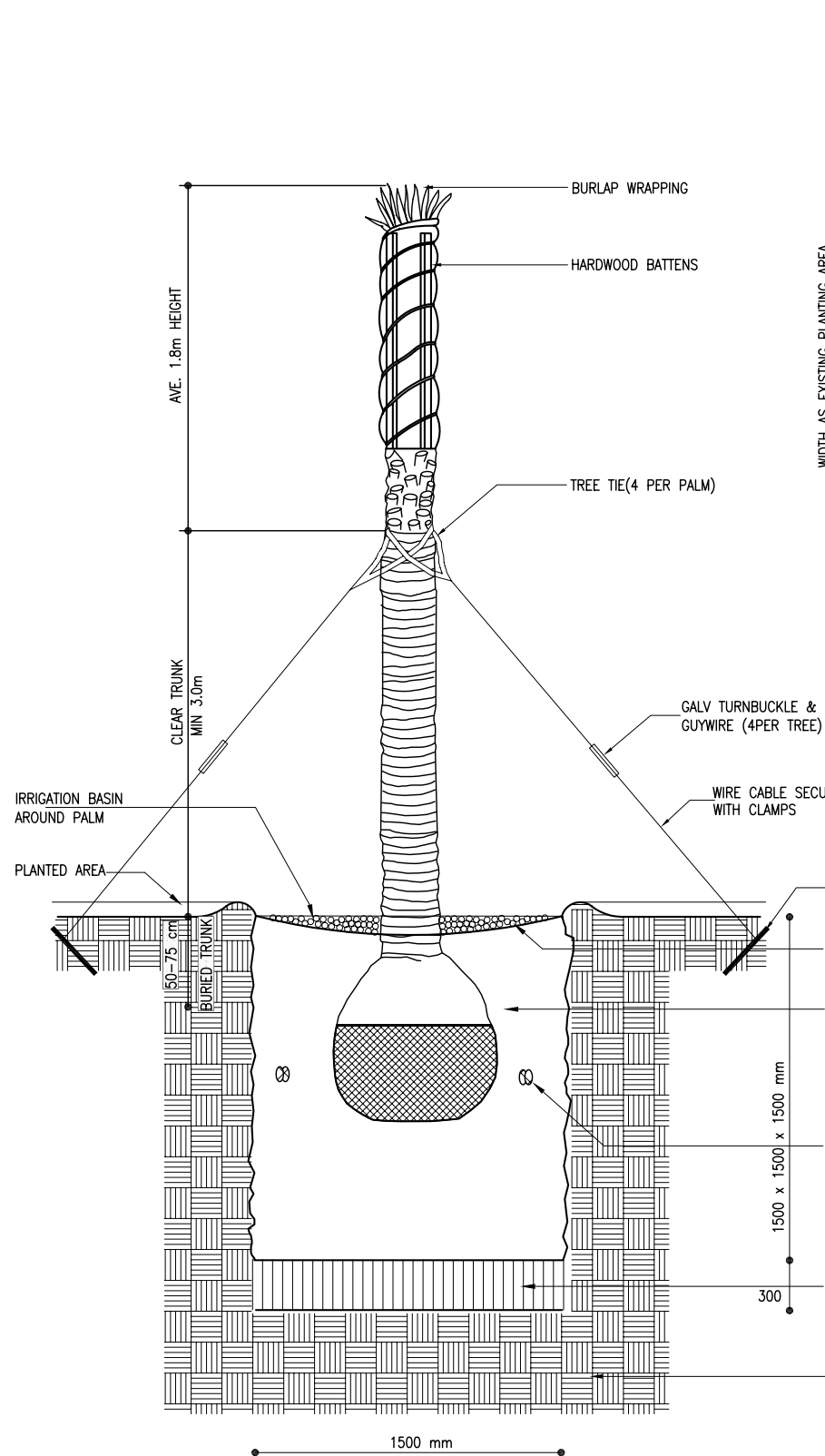
PALM PLANTING AND BRACING
