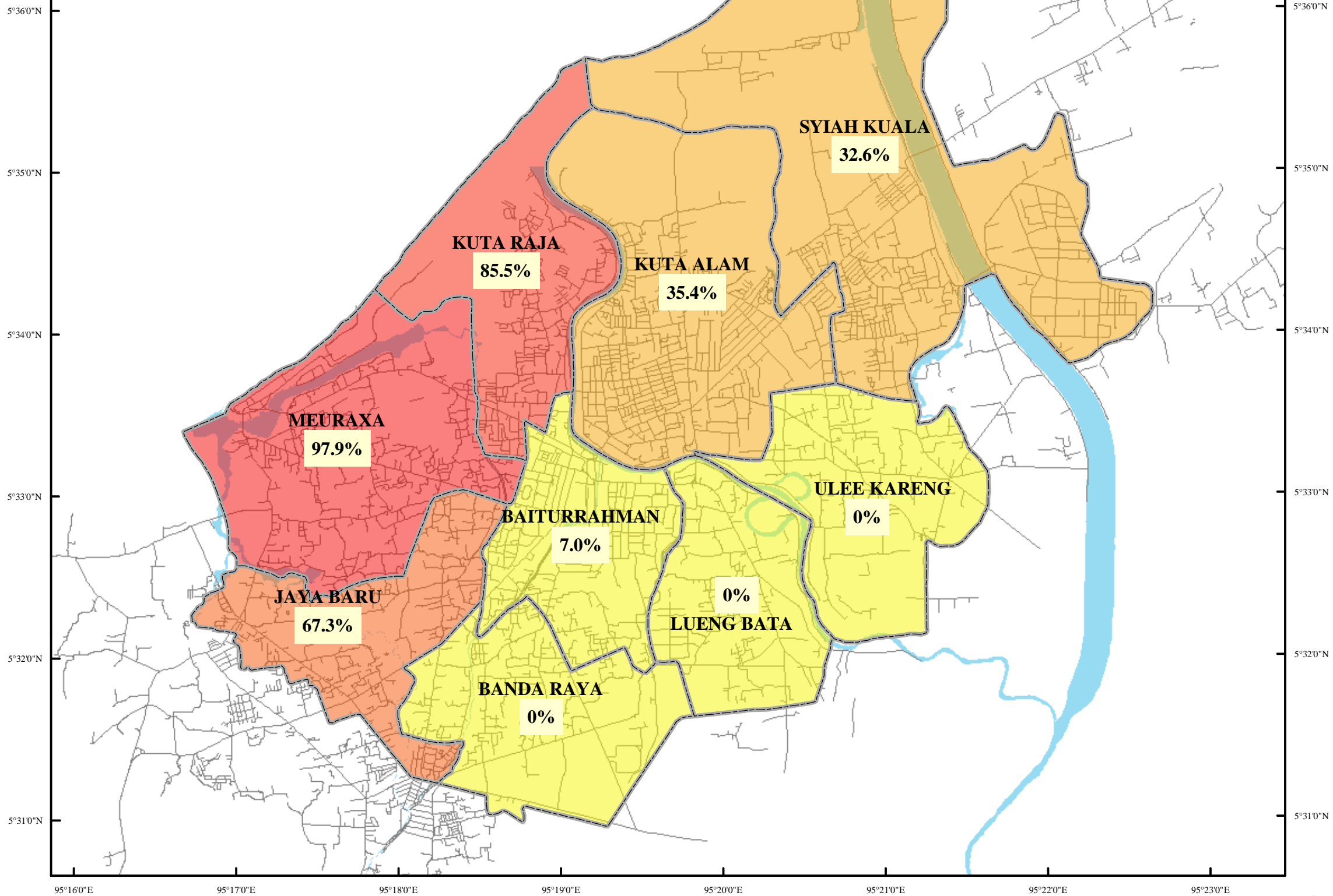
Damage Rate of Streets by Kecamatan
