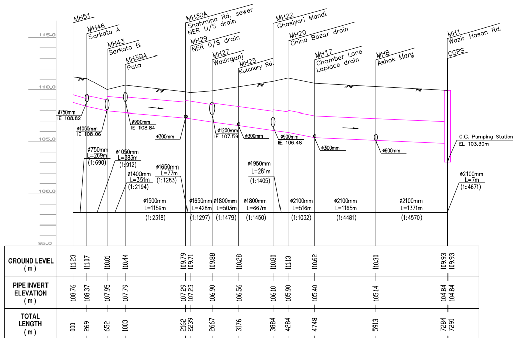
1a PROFILE CIS GOMTI TRUNK SEWER
