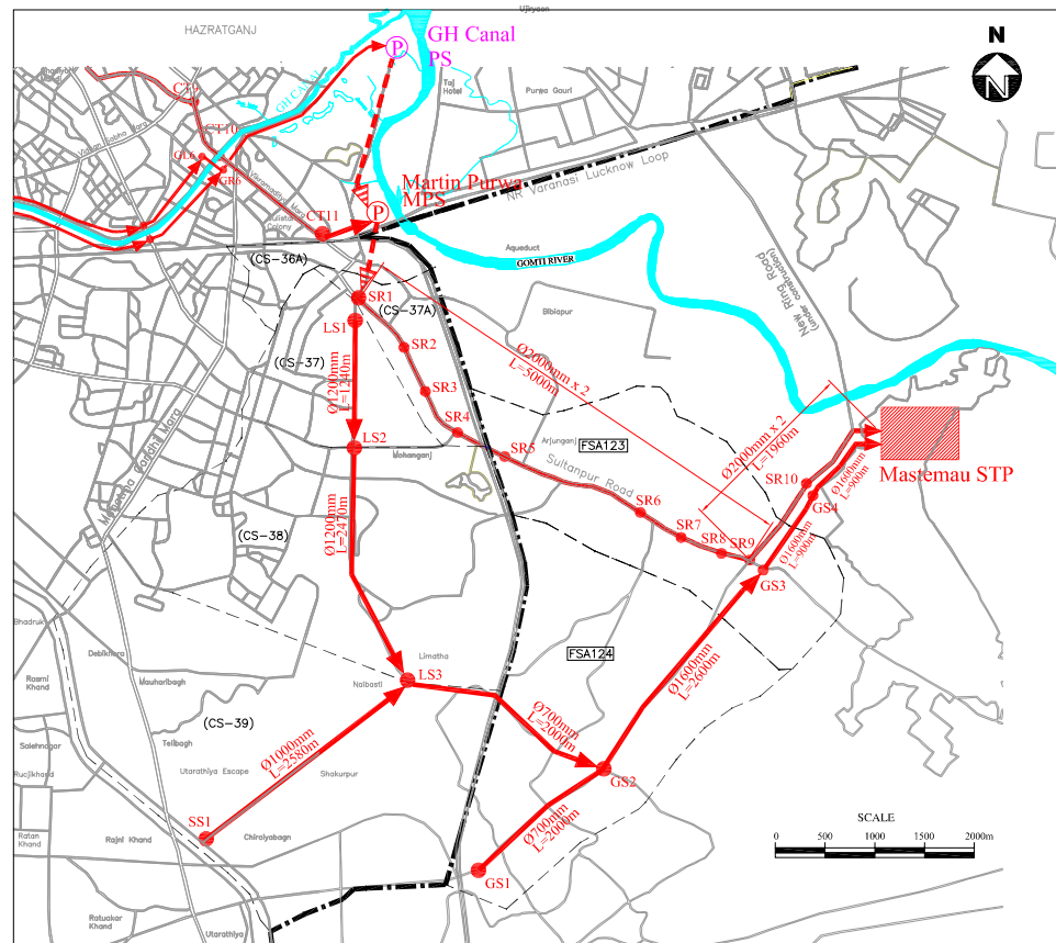
1 PLAN
