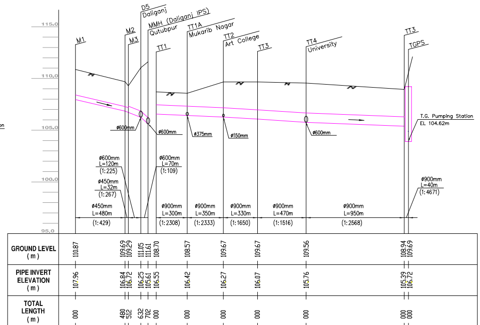
1b PROFILE TRANS GOMTI TRUNK SEWER
