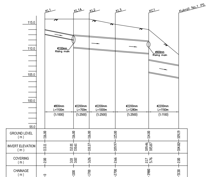
1c PROFILE KUKRAIL NALA INTERCEPTOR LEFT BANK (KL1-PS)
