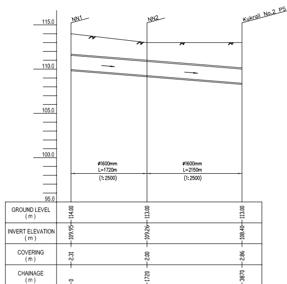
1a PROFILE MAHANAGAR SEWER (NN1-PS)
