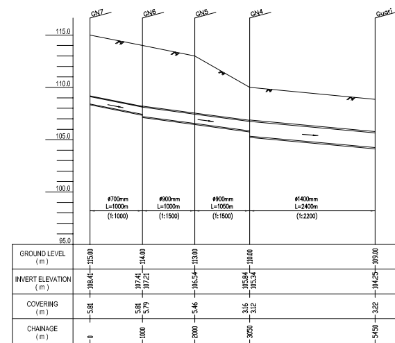
1g PROFILE GOMTI NAGAR NO.2 SEWER (GN7-PS)
