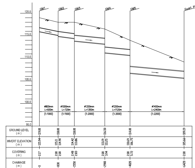
1i PROFILE GOMTI NAGAR MAIN SEWER (GM1-PS)
