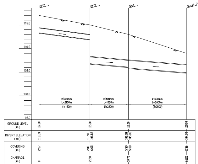
1f PROFILE GOMTI NAGAR NO.1 SEWER (GN3-PS)
