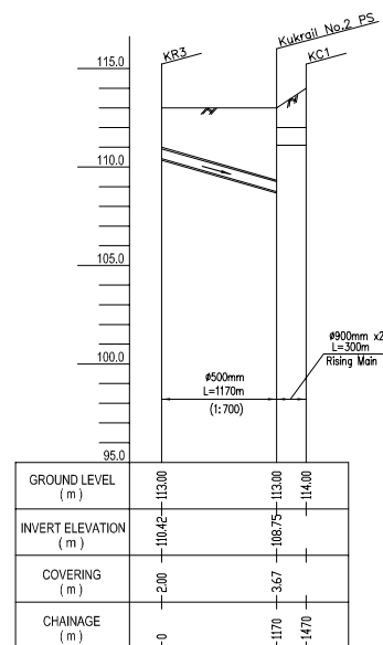
1b PROFILE KUKRAIL NALA INTERCEPTOR RIGHT BANK (KR3-KC1)
