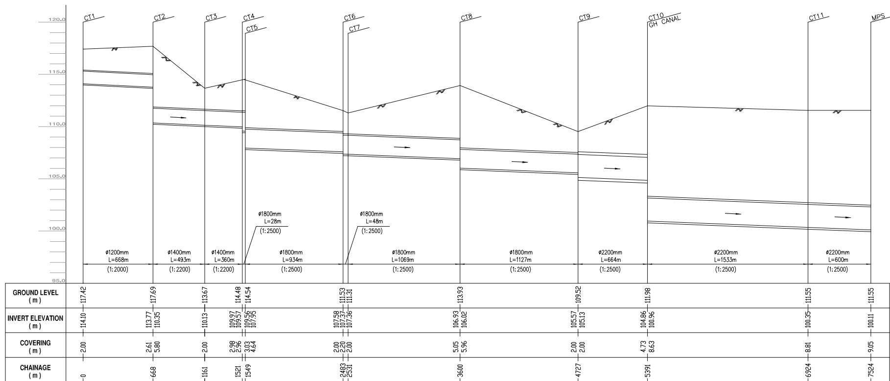
1 PROFILE CIS GOMTI RELIEF SEWER (CT1-STP)
