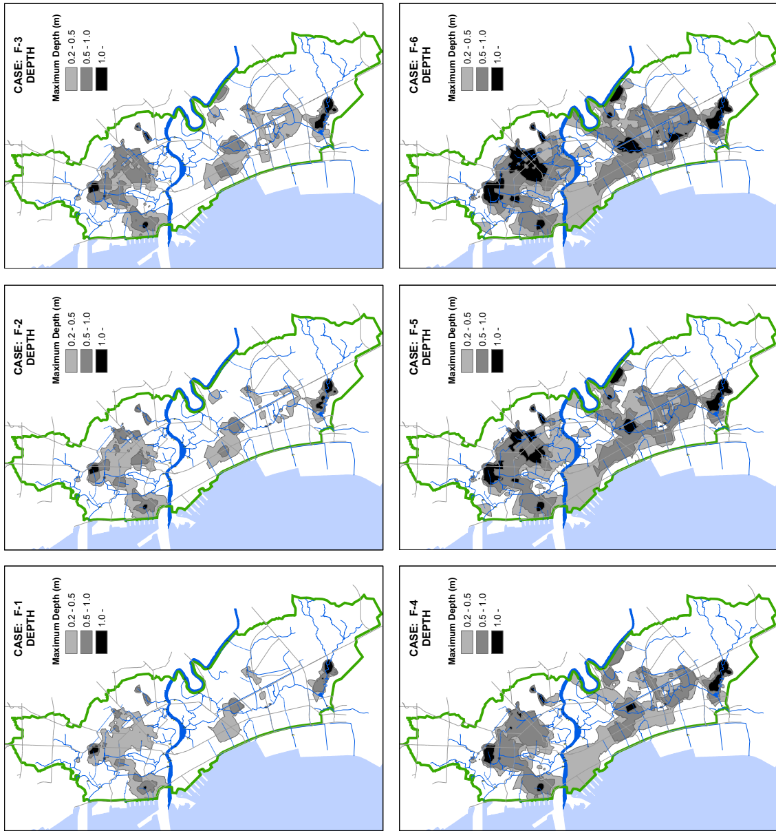
Figure D.7.1 Inundation Map of Depths and Durations for Different Cases (4/7)
