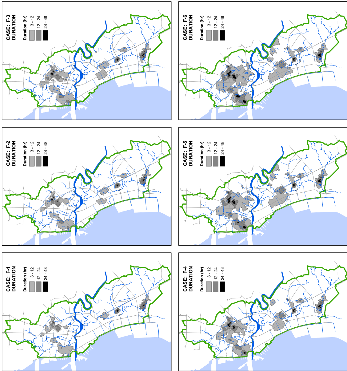
Figure D.7.1 Inundation Map of Depths and Durations for Different Cases (5/7)
