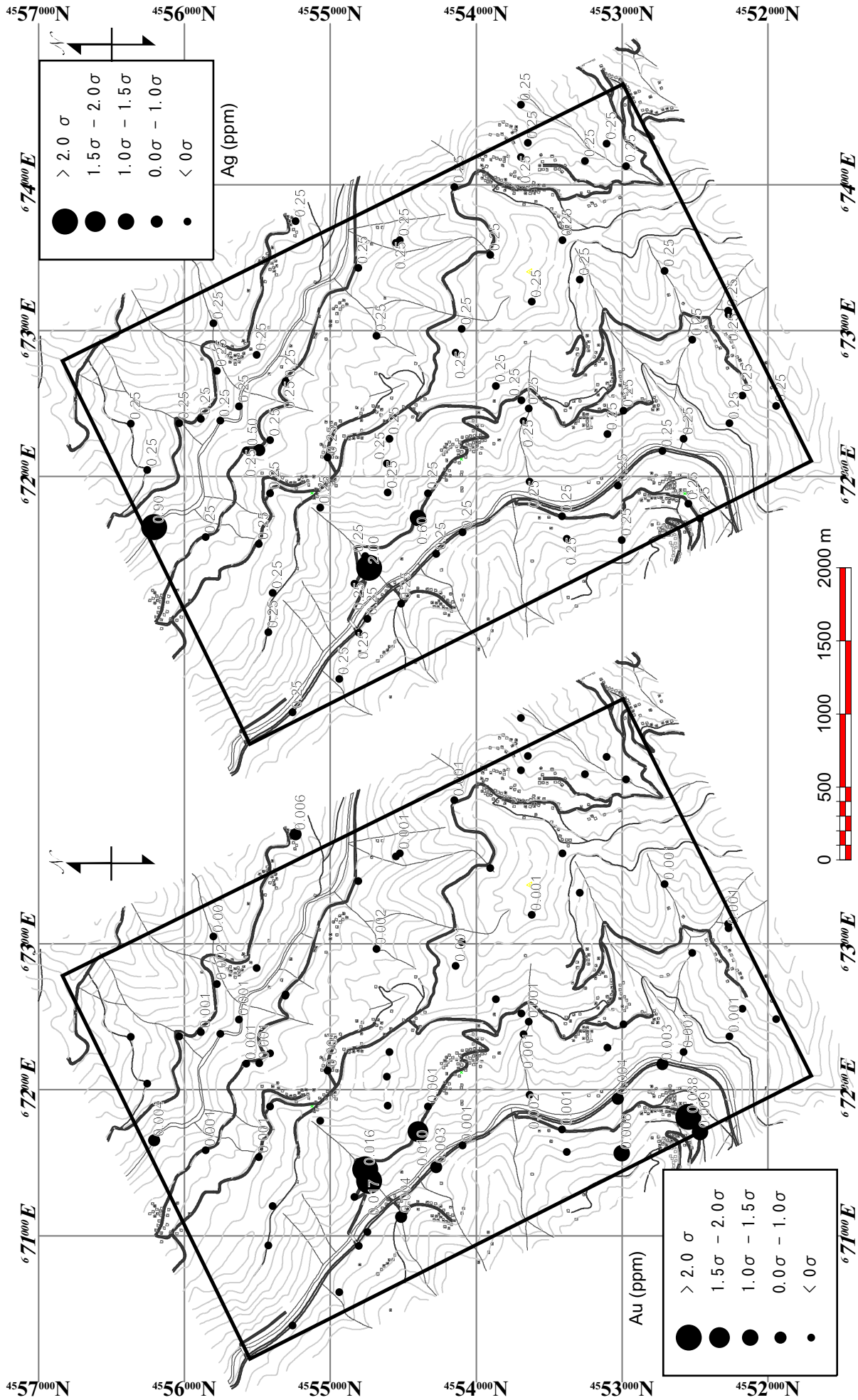
Appendix 6 Distribution Map of Au and Ag by Rock Specimens
