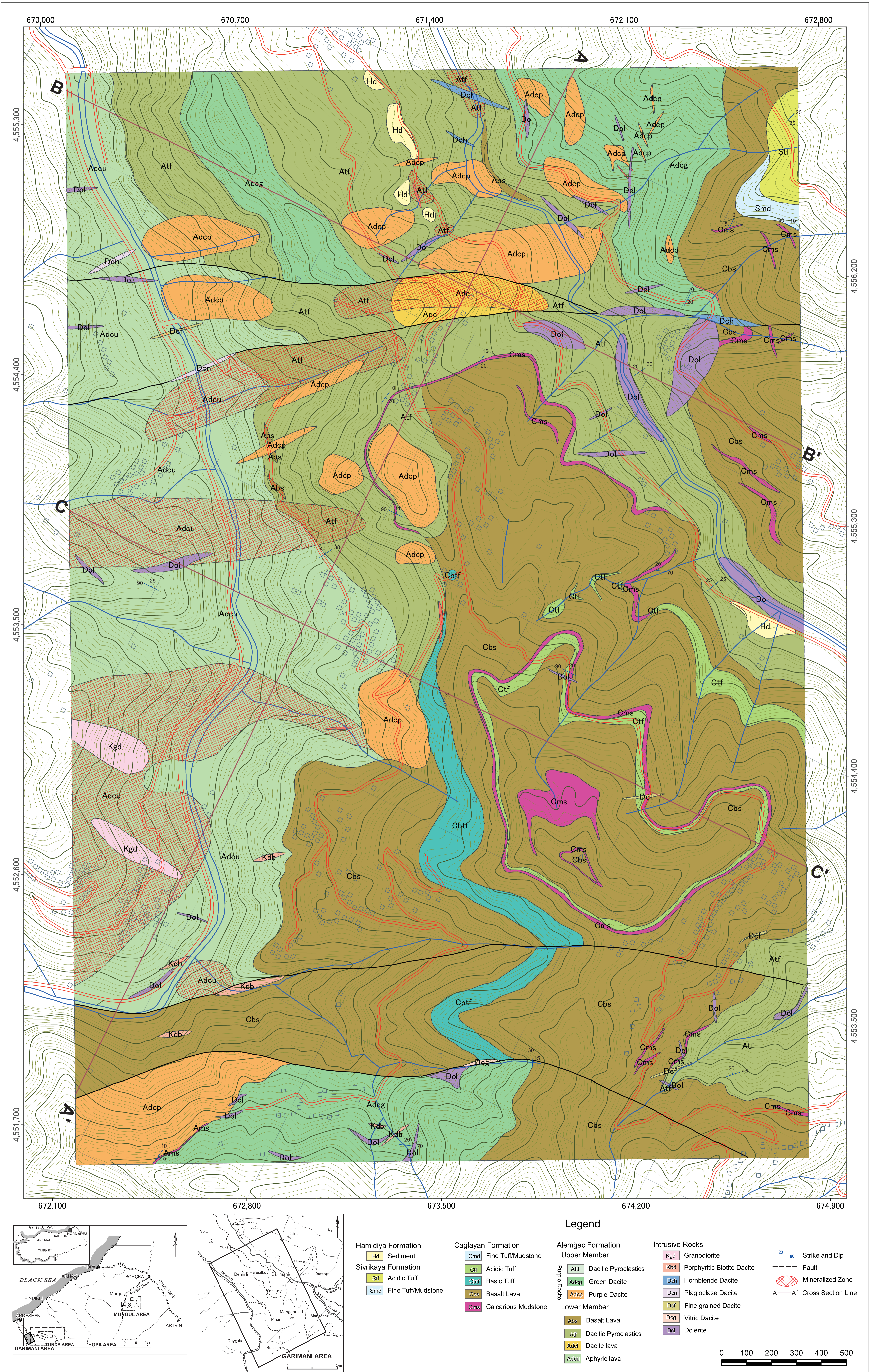
Geological Map of the Garimani Area
