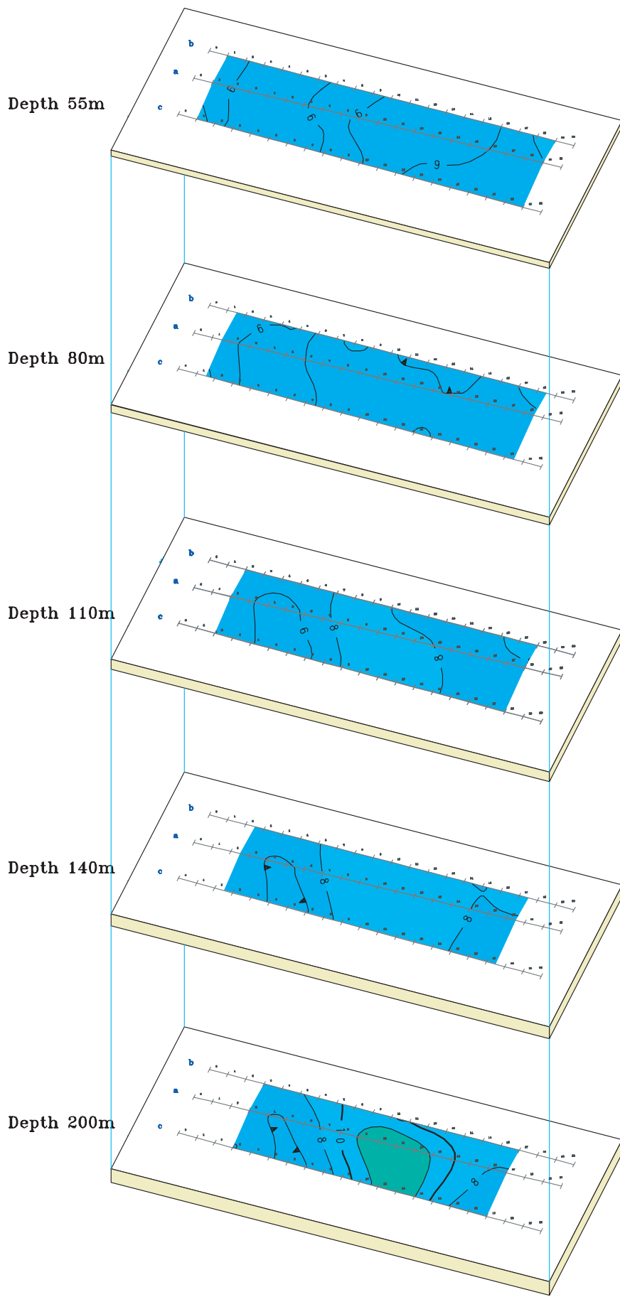
Fig.II-4-2-7 2D Analysis plane map of chargeability at Khefawna area
