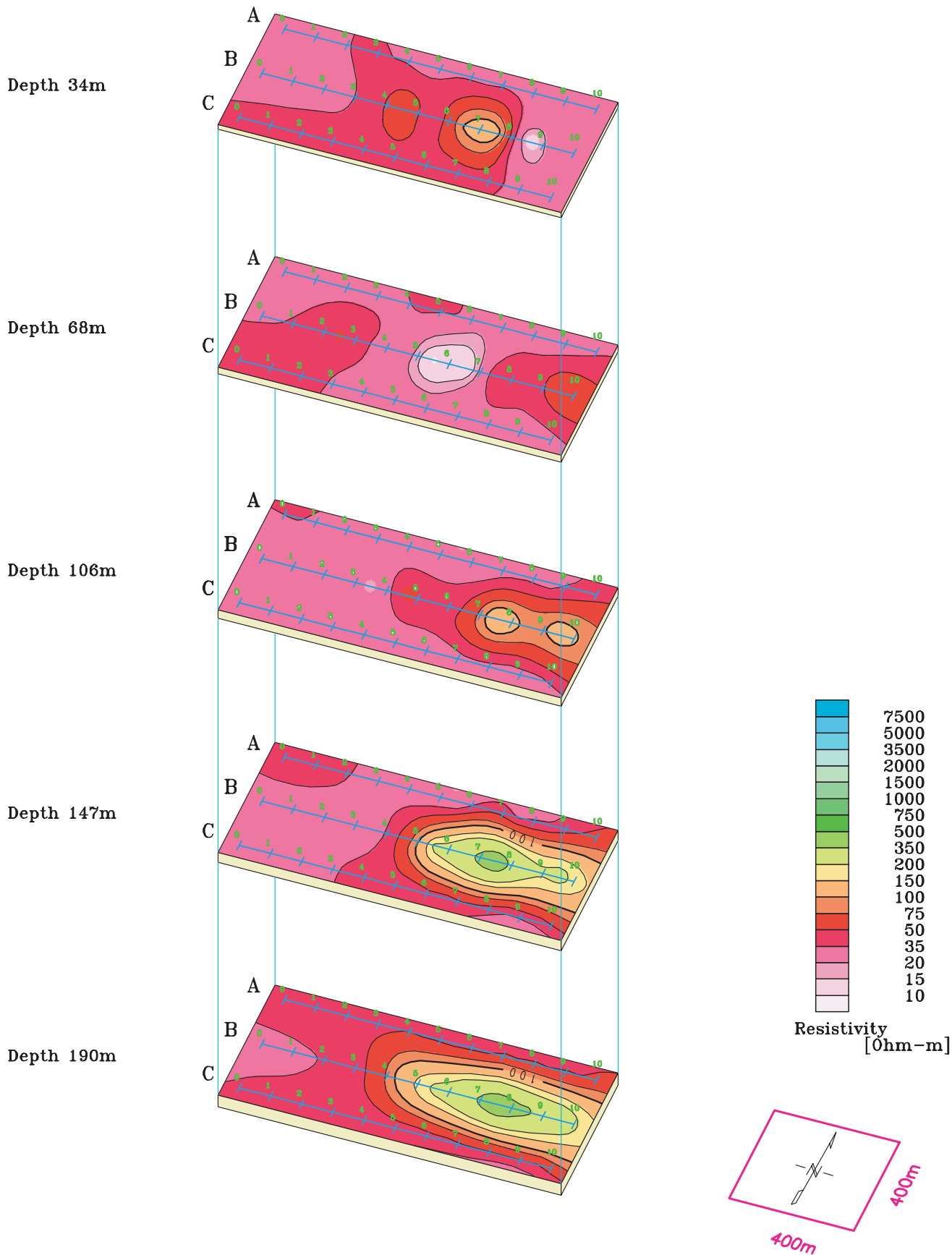
Fig.II-4-1-12 2D Analysis plane map of resistivity (MJTK-IP-6)
