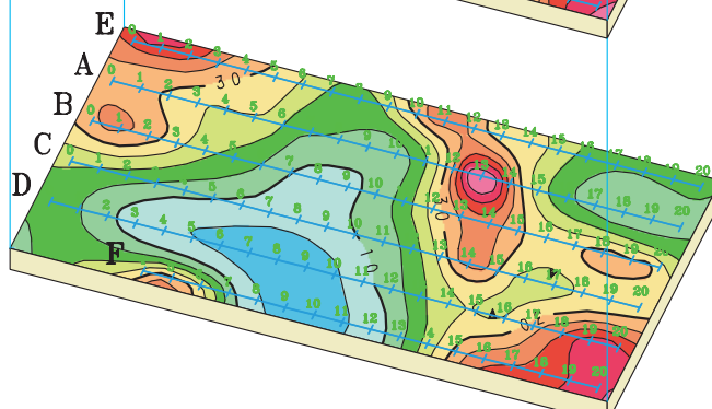
Fig.II-4-1-8 2D Analysis plane map of metal factor (MJTK-IP-1)
