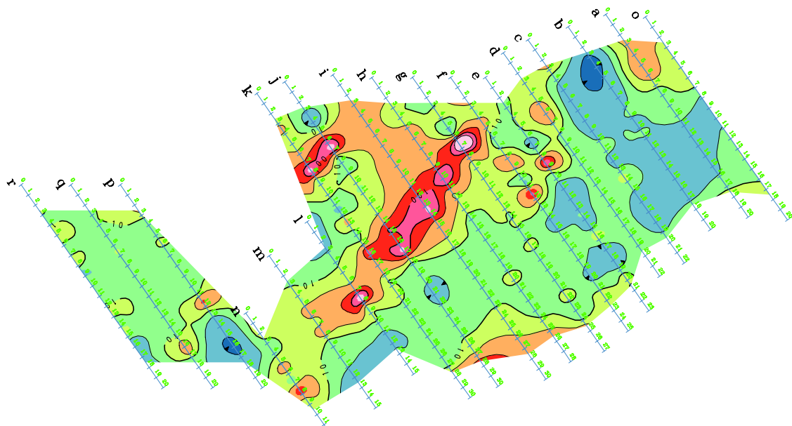
Fig.II-2-1-61 2D Analysis plane map at Azzouz area (140m depth)
