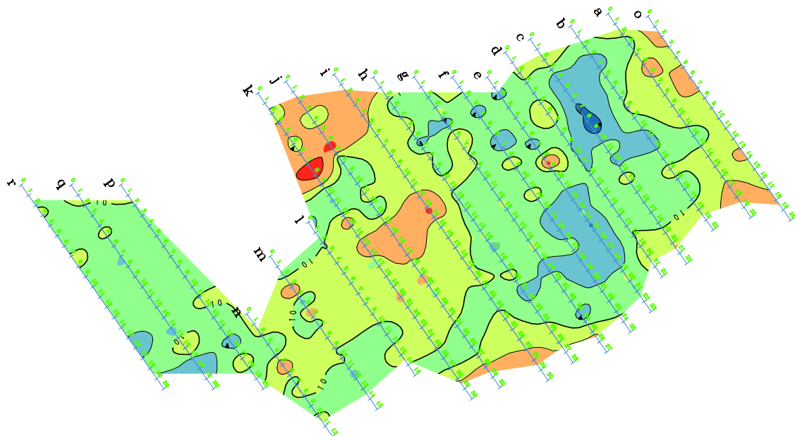
Fig.II-2-1-59 2D Analysis plane map at Azzouz area (80m depth)
