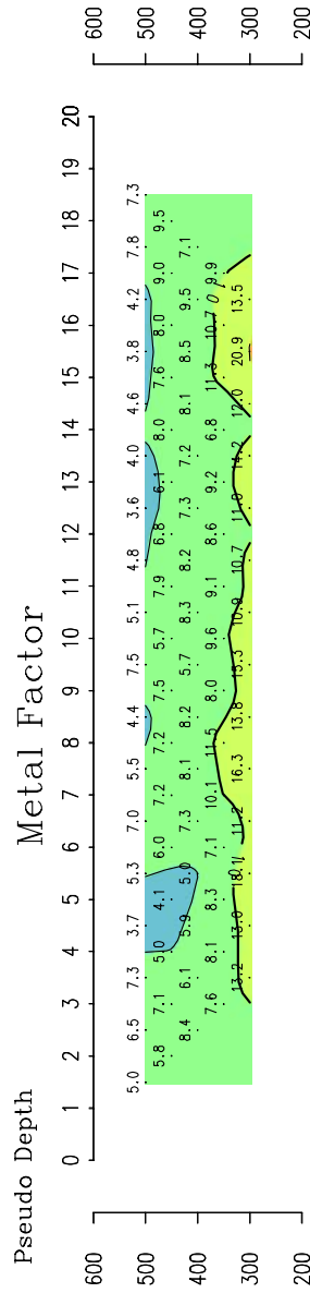
Fig.II-2-1-29 IP pseudo-sections at Harch area (a line)
