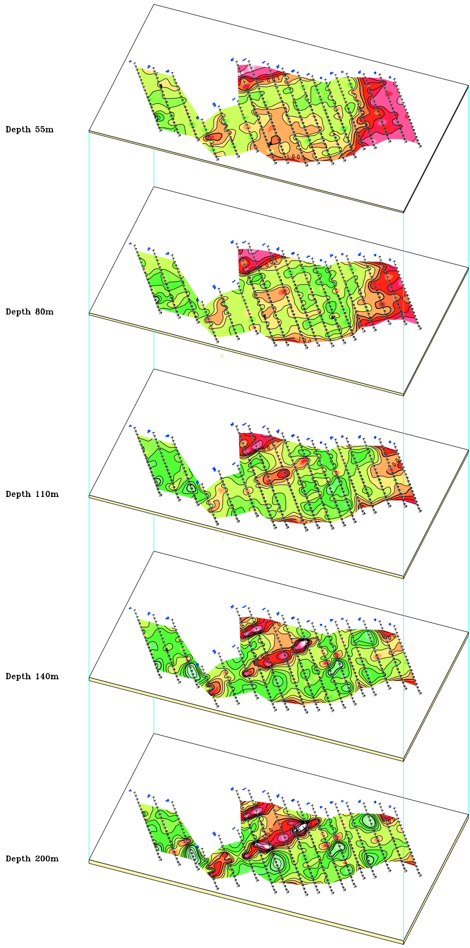
Fig.II-2-1-63 2D Analysis plane map of resistivity at Azzouz area
