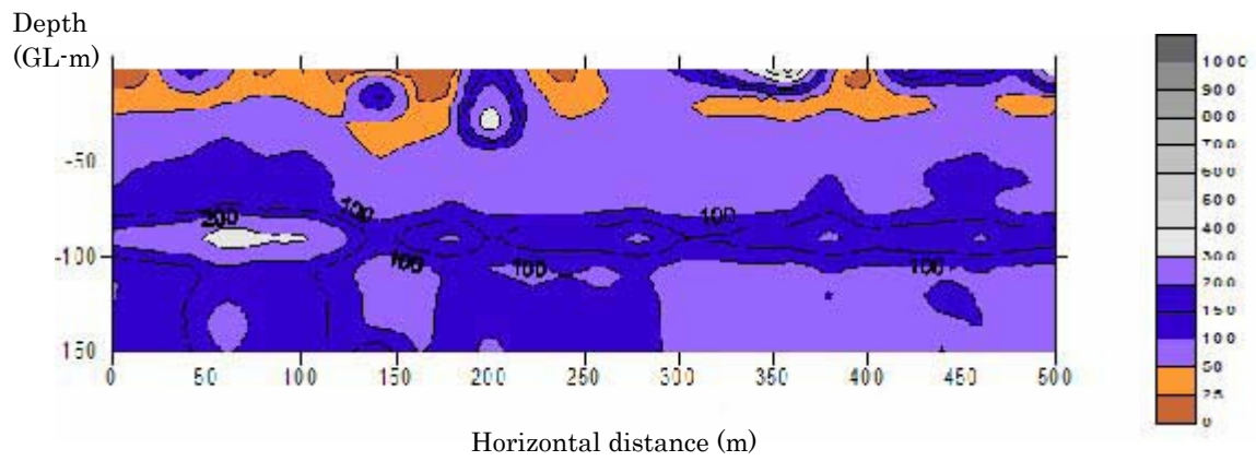
2-D Electric Sounding
