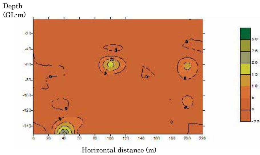
IP (Induced Polarization) Method Sounding
