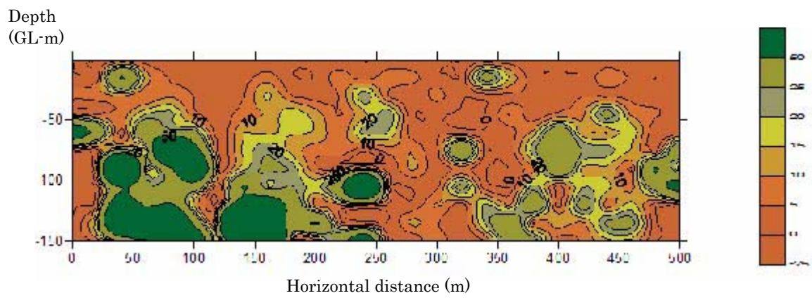
IP (Induced Polarization) Method Sounding
