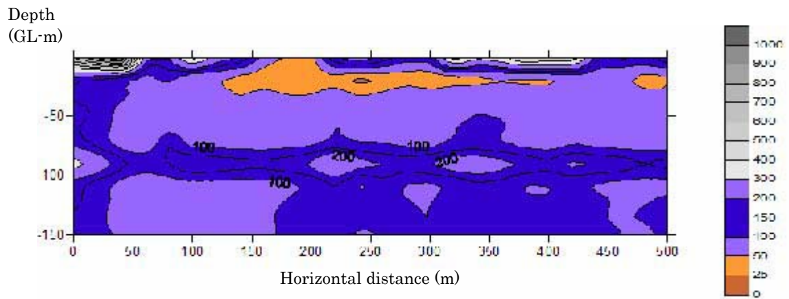
2-D Electric Sounding
