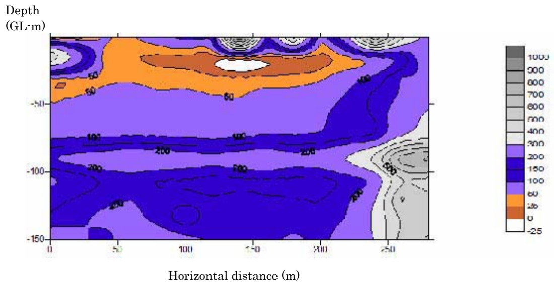
2-D Electric Sounding
