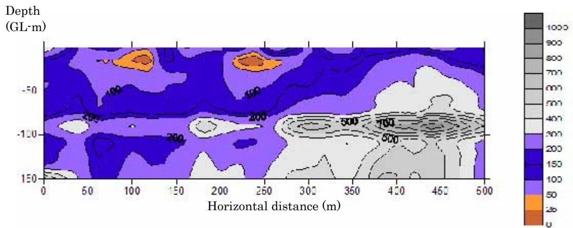
2-D Electric Sounding
