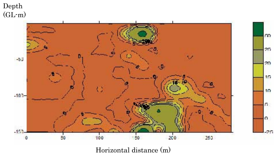
IP (Induced Polarization) Method Sounding
