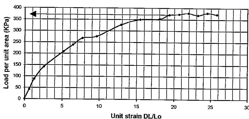
Unconfined compressive curve
