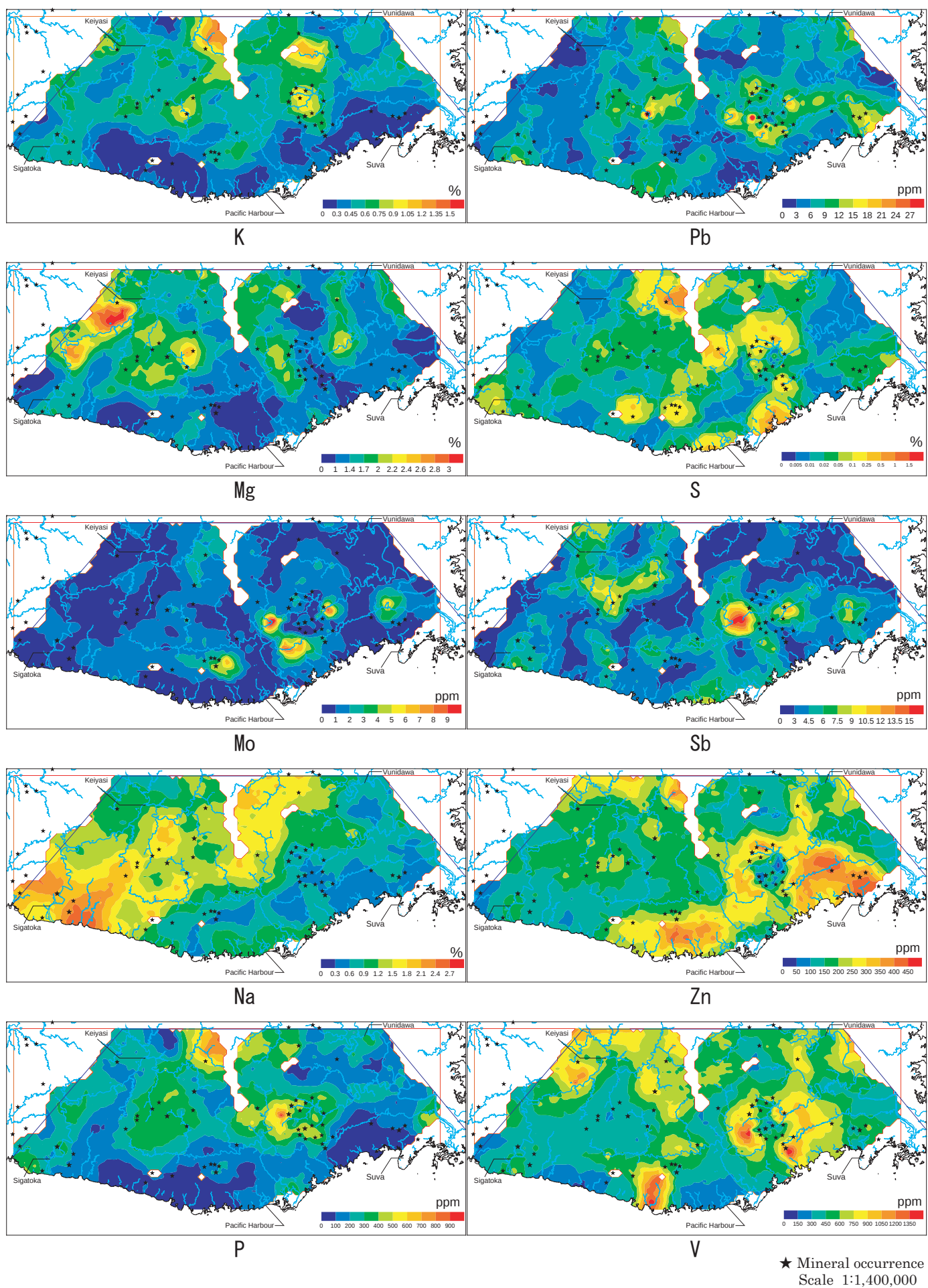
Fig.3-2-1. Geochemical map of the stream sediments (2)
