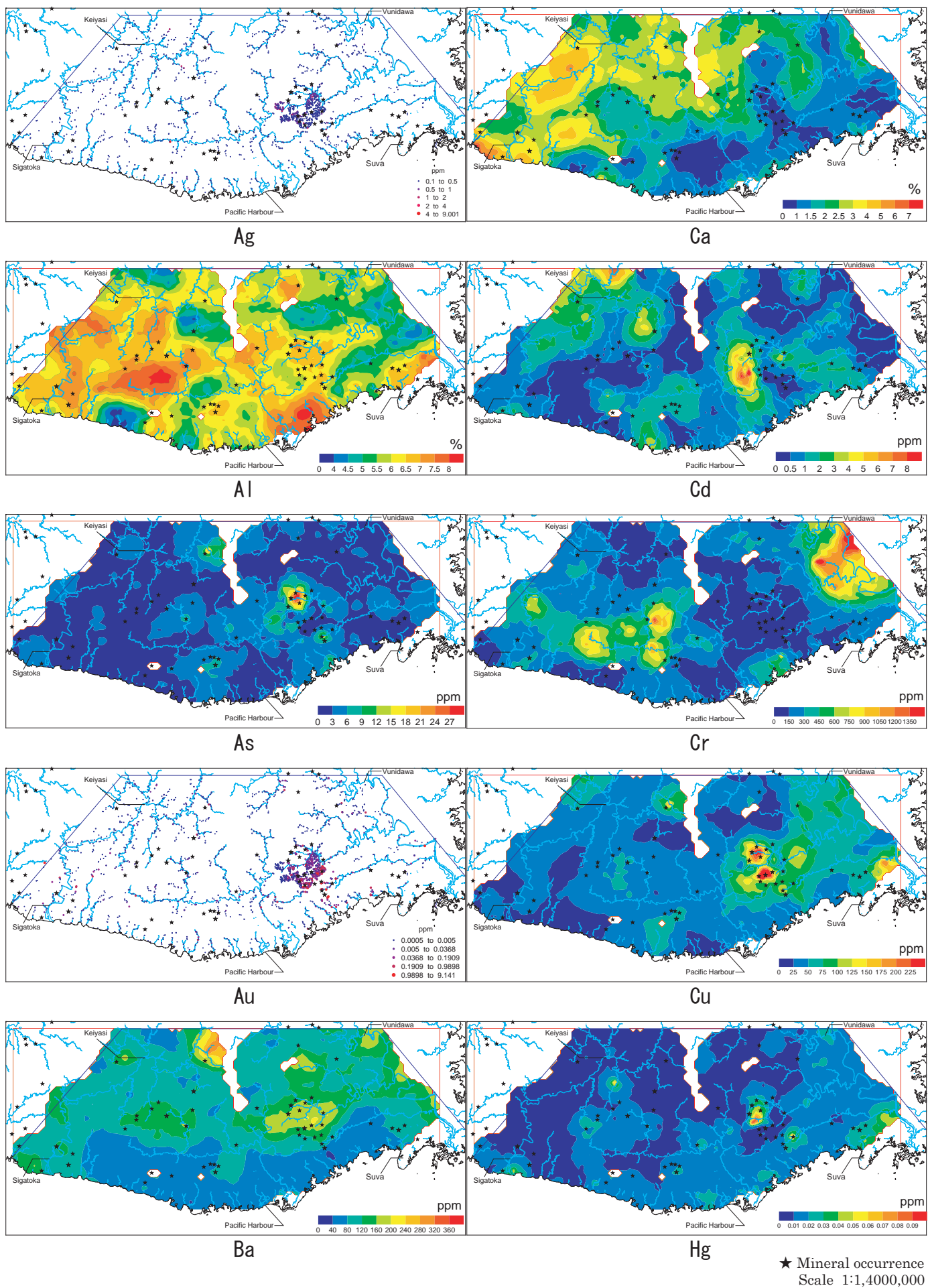
Fig.3-2-1. Geochemical map of the stream sediments (1)
