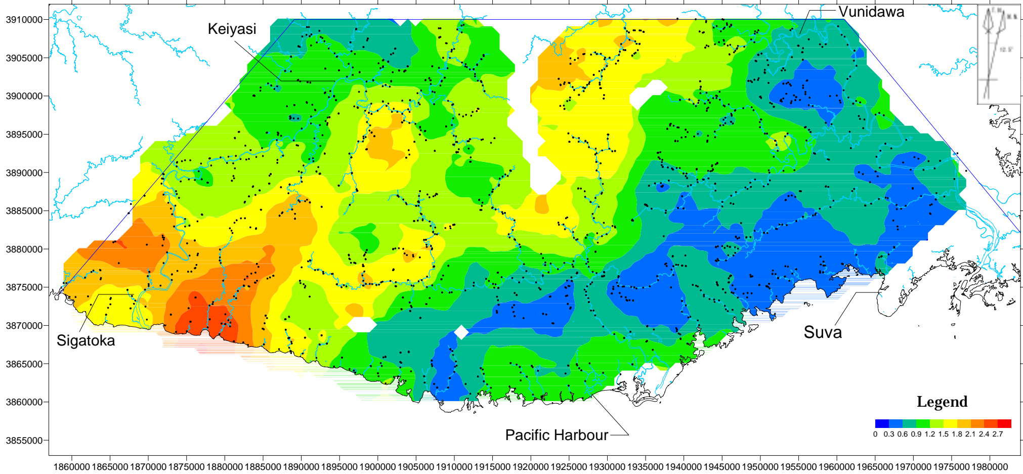
Figure II-1-3-(14) Geochemical map of Na (%) in stream sediment samples (1:500,000)
