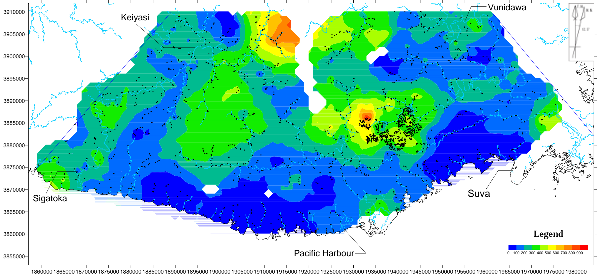
Figure II-1-3-(15) Geochemical map of P (ppm) in stream sediment samples (1:500,000)
