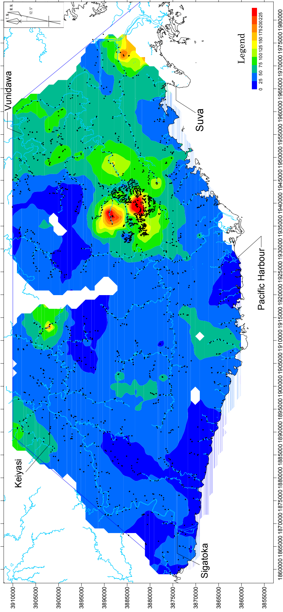
Figure II-1-3-(9) Geochemical map of Cu (ppm) in stream sediment samples (1:500,000)
