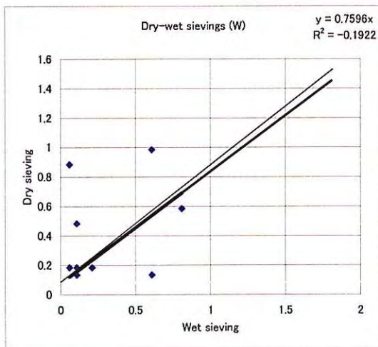
Fig. 3-2 Comparison of Sampling Methods of Stream Sediments (3/3)
