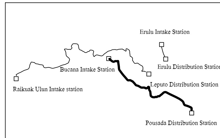
Bucana Intake Station \phi 100 Raw Water Main Pousada Distribution Station
