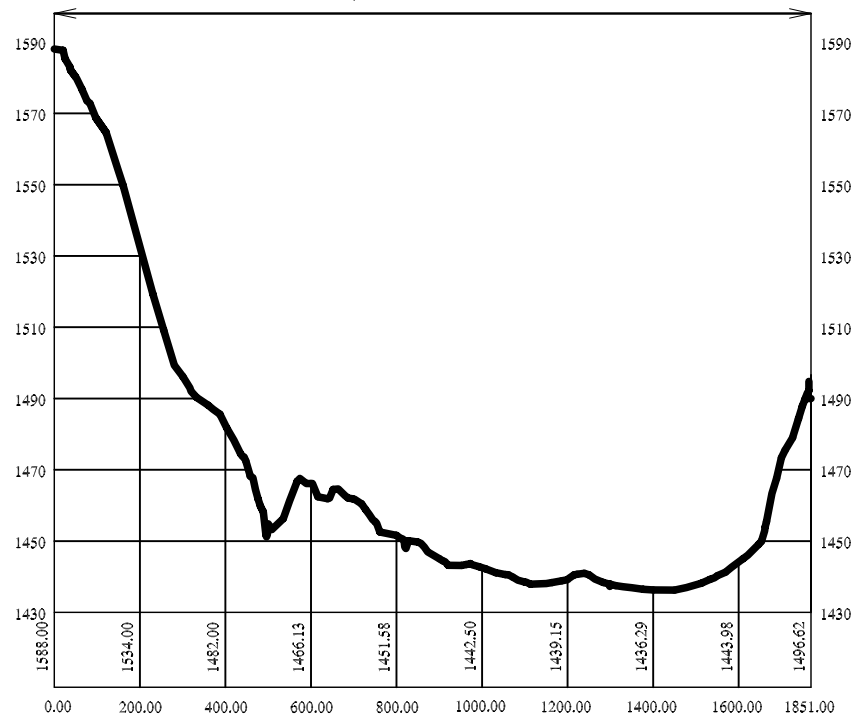
Bucana Intake Station \phi 100 Raw Water Main Pousada Distribution Station
