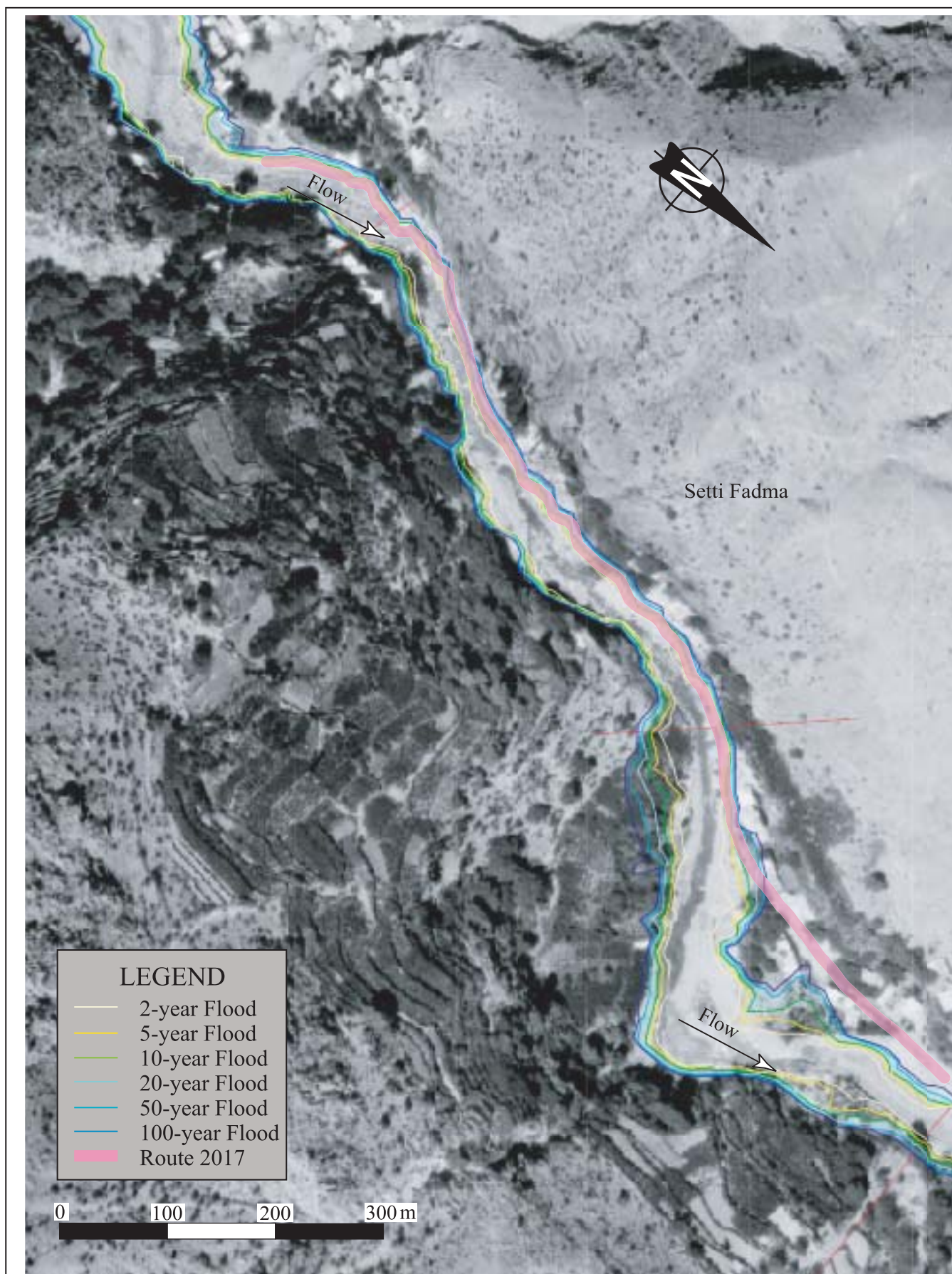
Fig. D.3.7(5/5) FLOOD MAP OF OURIKA RIVER (AROUND SETTI FEDMA VILLAGE)
