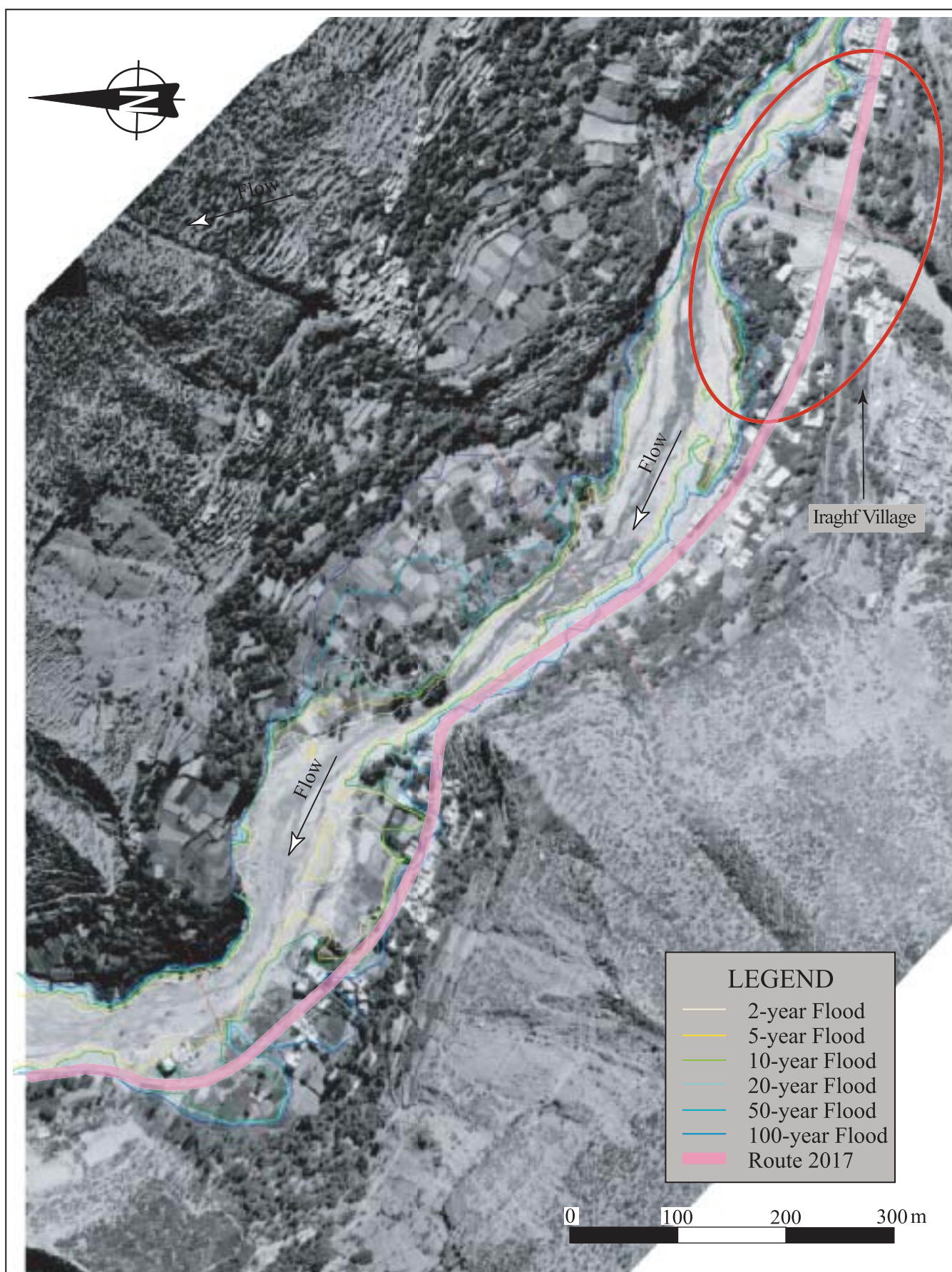
Fig. D.3.7 (3/5) FLOOD MAP OF OURIKA RIVER (DOWNSTREAM OF IRAGHF VILLAGE)
