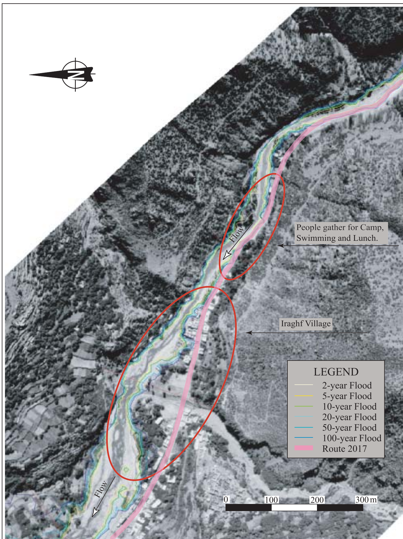
Fig. D.3.7 (4/5) FLOOD MAP OF OURIKA RIVER (UPSTREAM OF IRAGHF VILLAGE)
