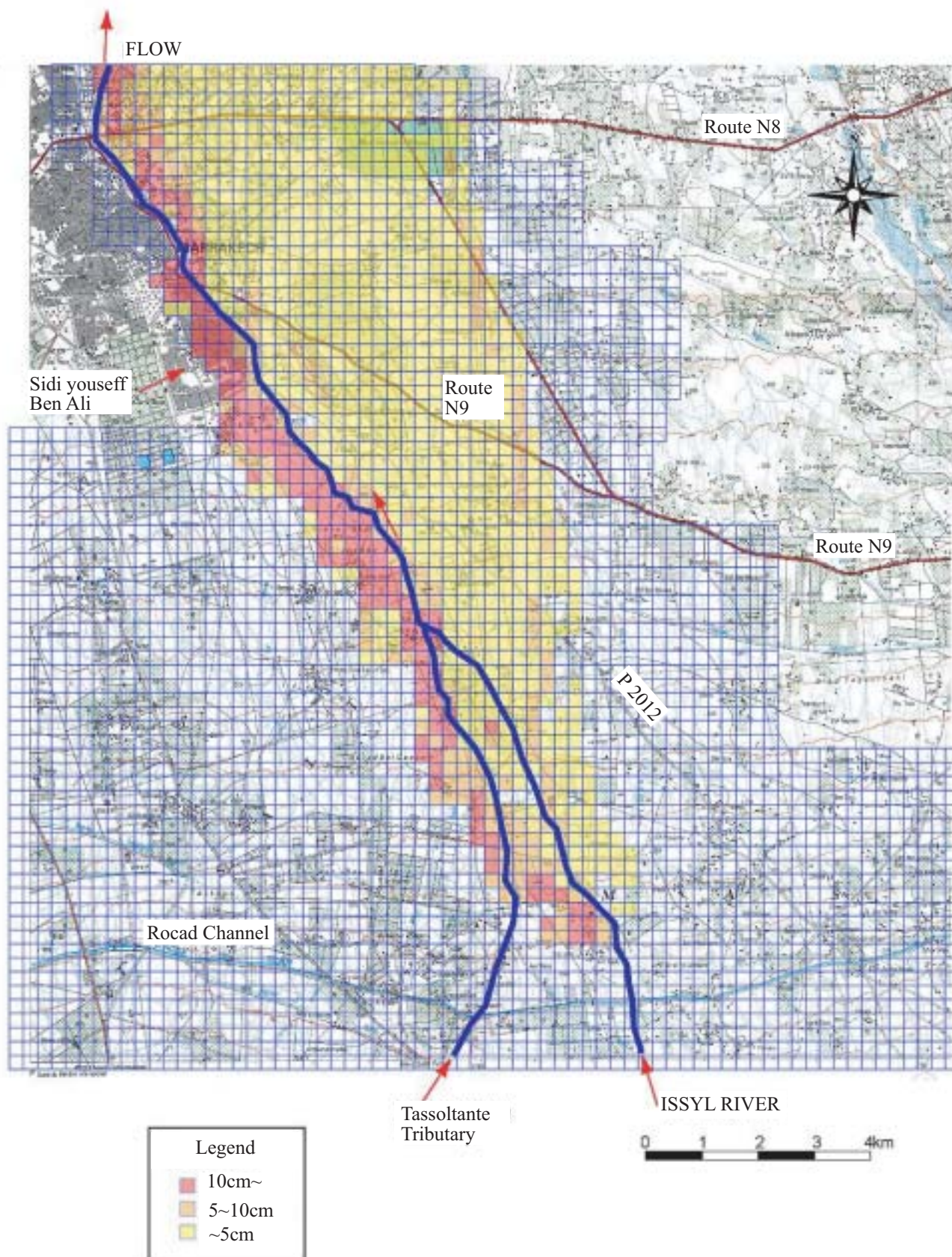
Fig. 3.2.22 FLOOD MAP OF ISSYL RIVER (100 YEAR FLOOD)
