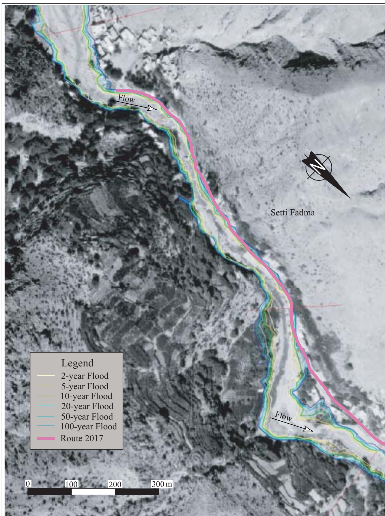
Fig. 3.2.18(5/5) FLOOD MAP OF OURIKA RIVER (AROUND SETTI FADMA VILLAGE)
