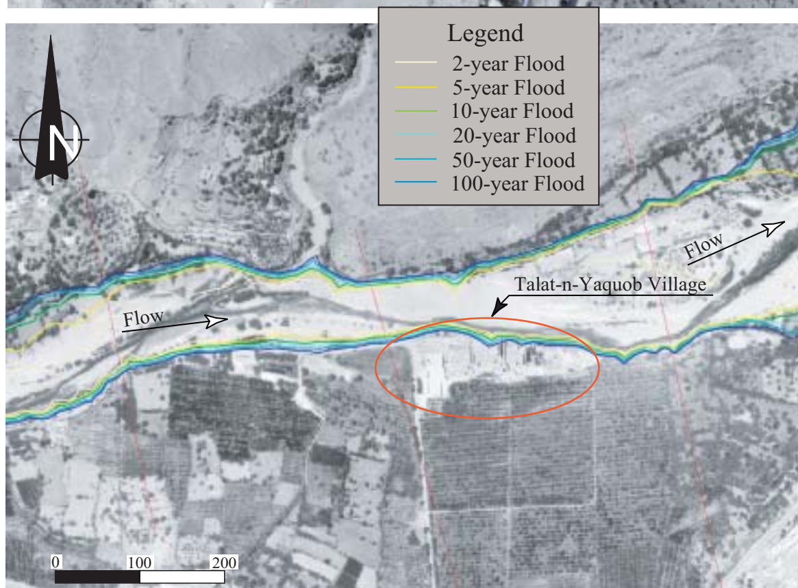
Fig. 3.2.14(2) FLOOD MAP OF N'FIS RIVER (AROUND IJOUKAK, TALAT- N-YAQUOB VILLAGE)
