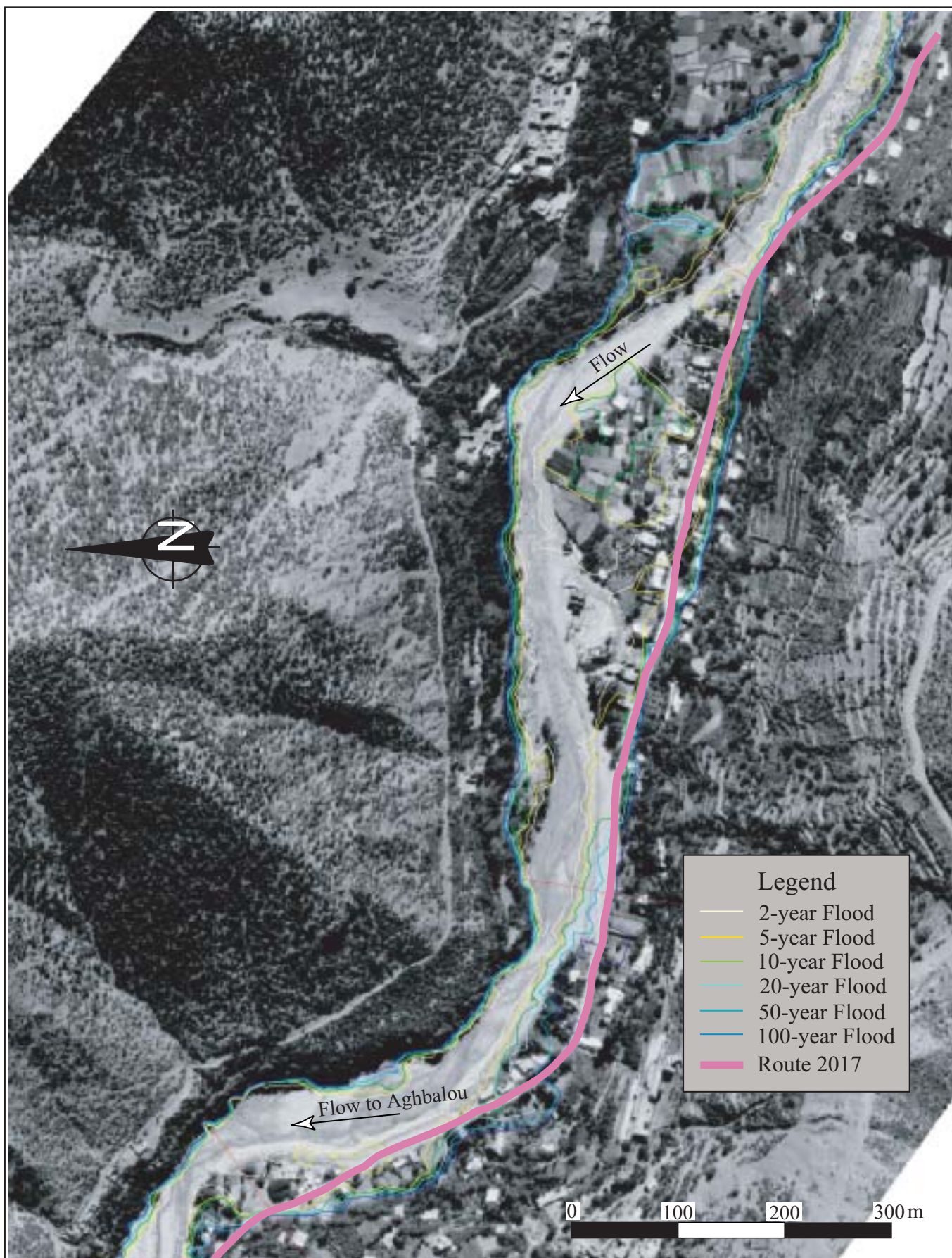
Fig. 3.2.18(2/5) FLOOD MAP OF OURIKA RIVER (UPSTREAM OF AGHBALOU)
