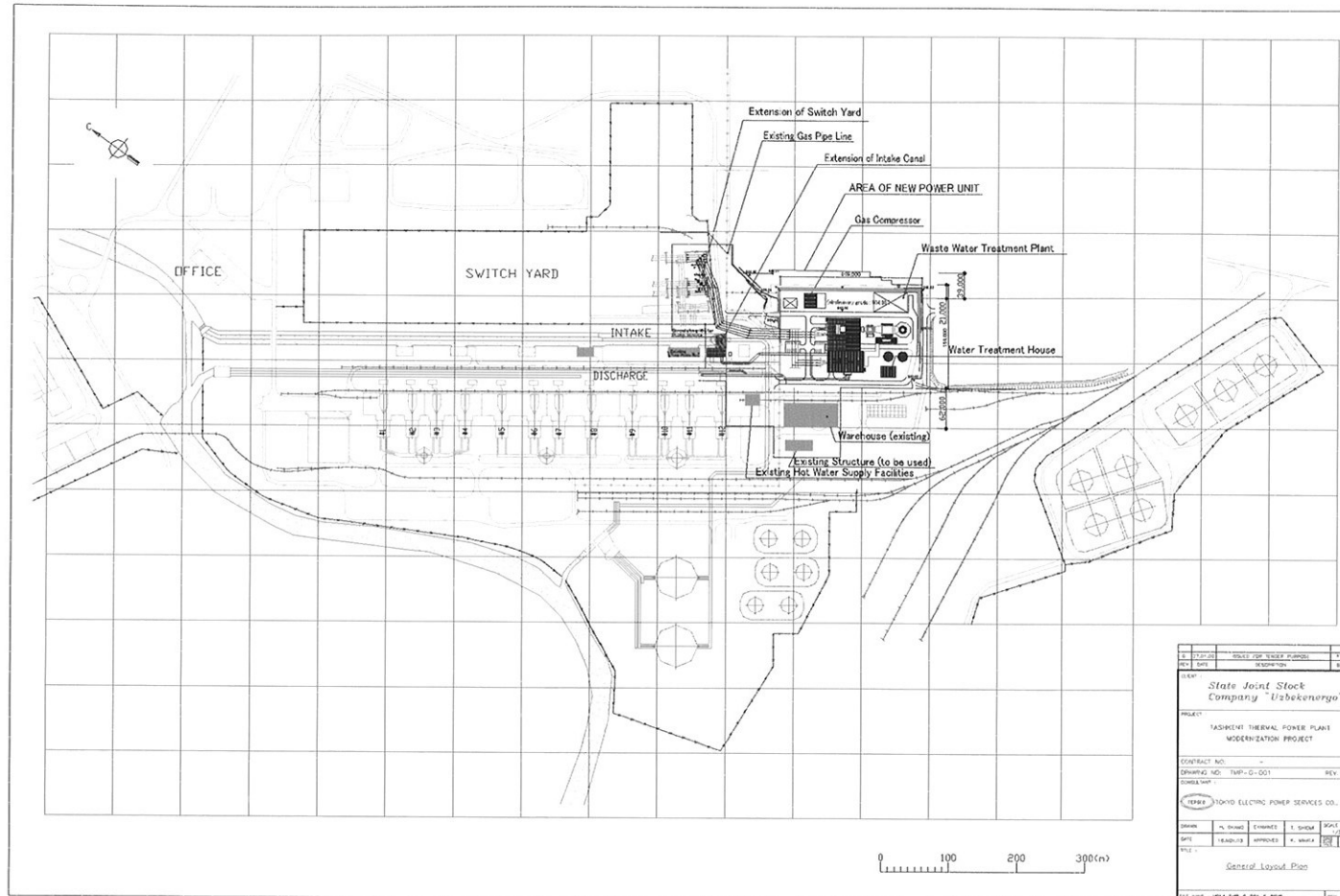
Site Layout Plan of Tashkent Thermal Power Station (After Modernization)
