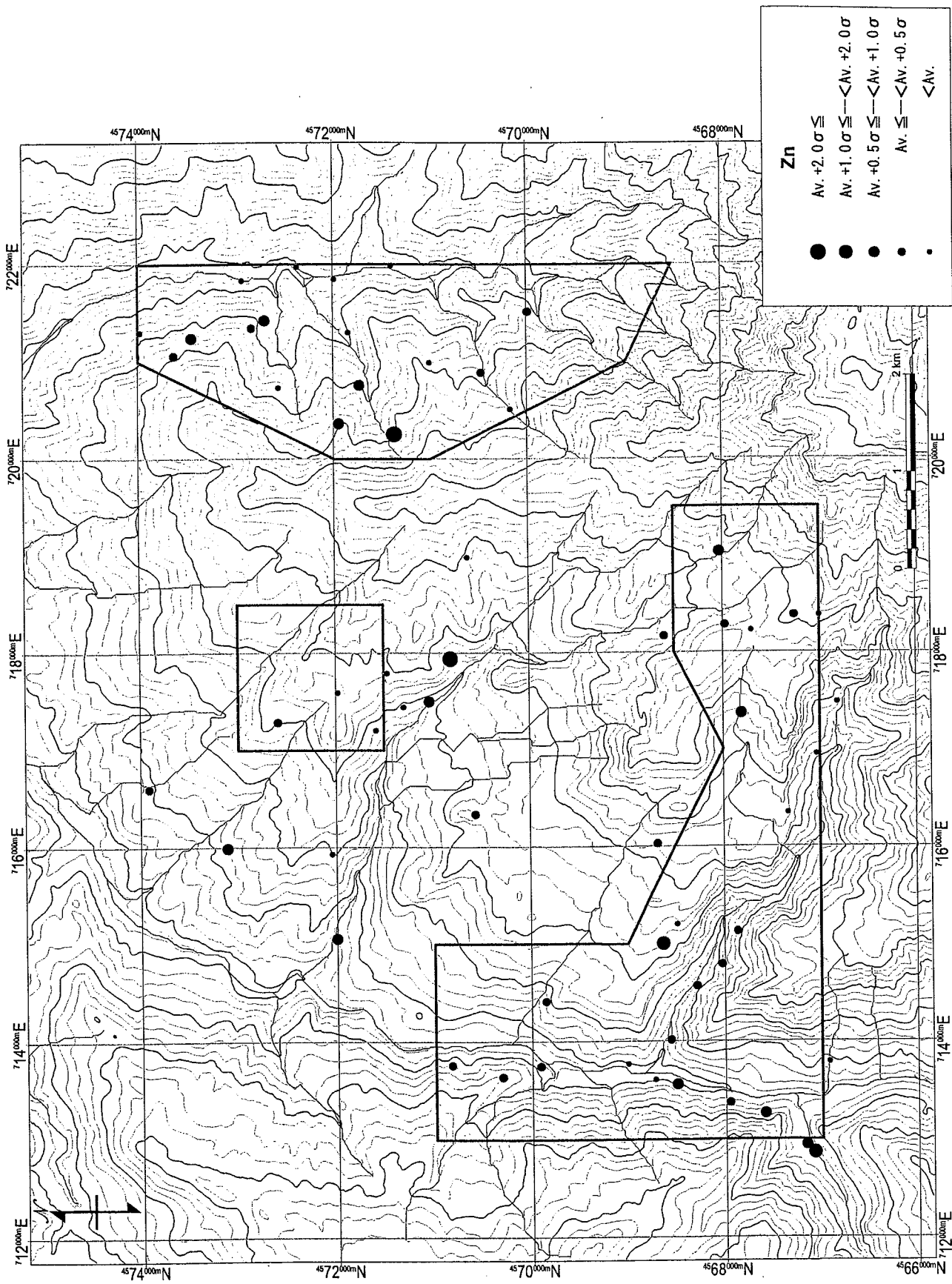
Appendix 7 Distribution Map of Zn by Rock Specimens (Murgul Area)
