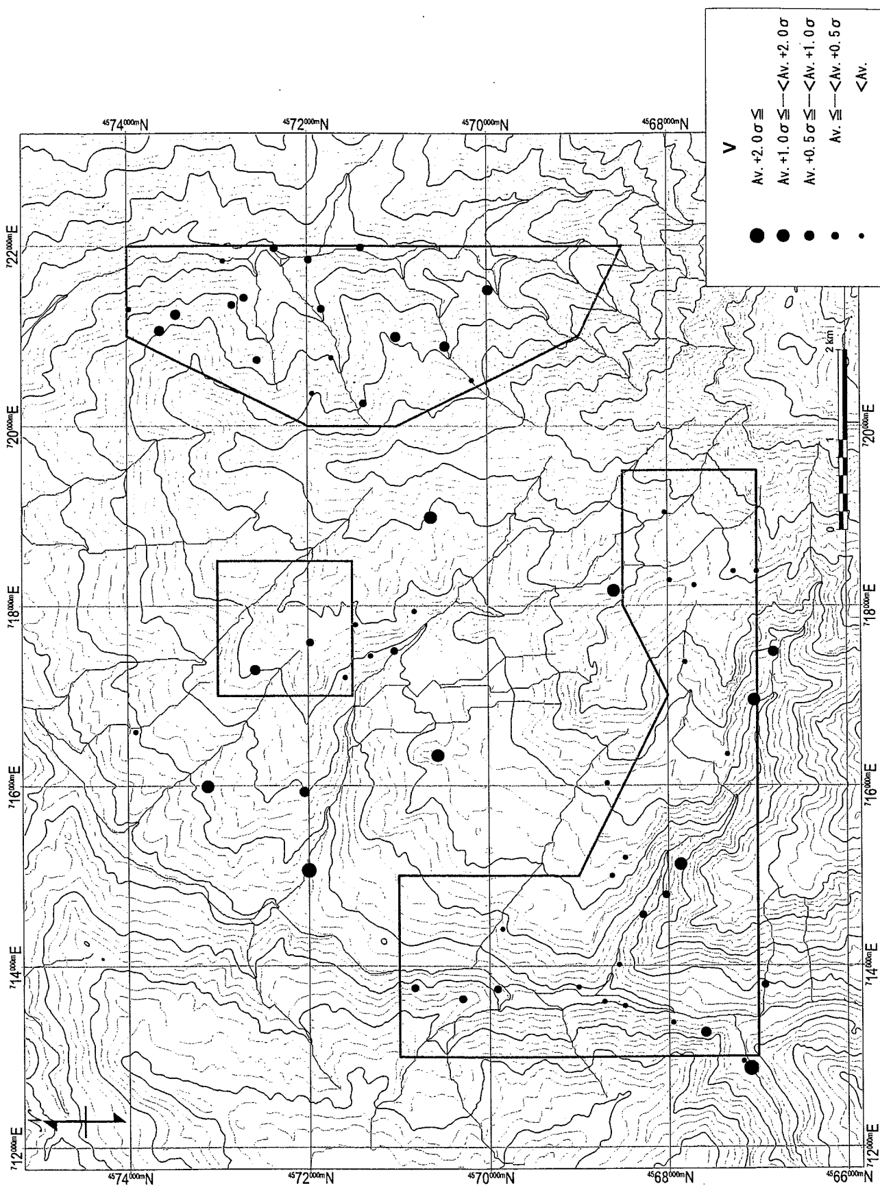
Appendix 7 Distribution Map of V Rock Specimens Murgul Area)
