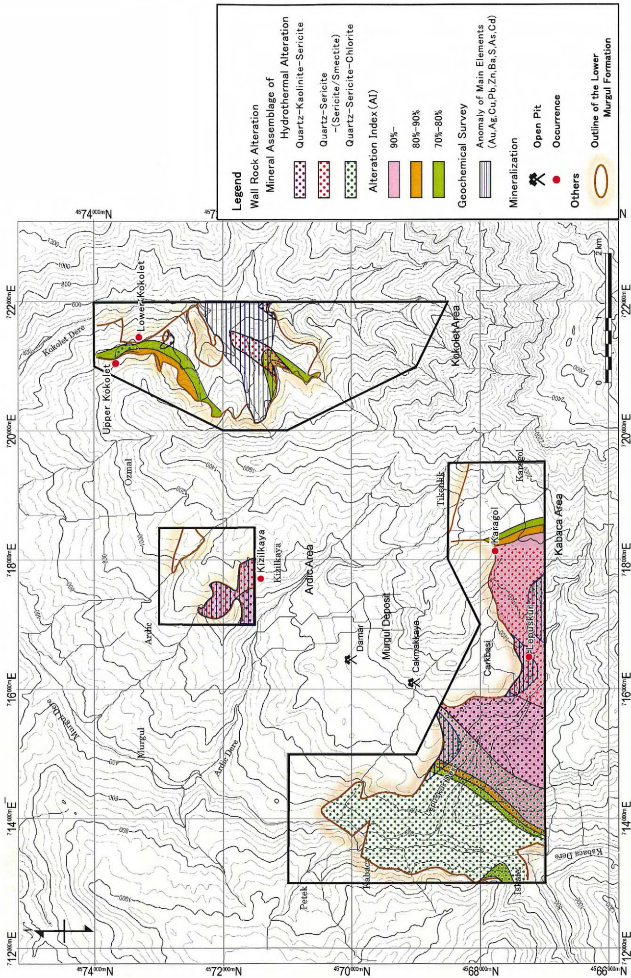
Fig. III-2 The Integrated Interpretation Map of the Murgul Area
