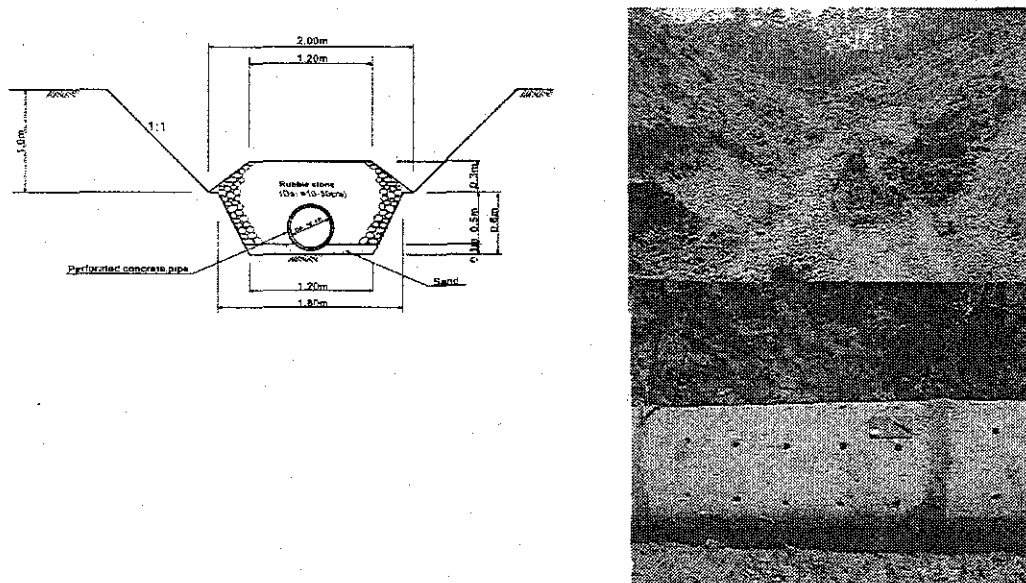
Figure H.2-5: Leachate Collection Facility
