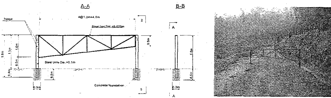
Figure H.2-15: Gate
