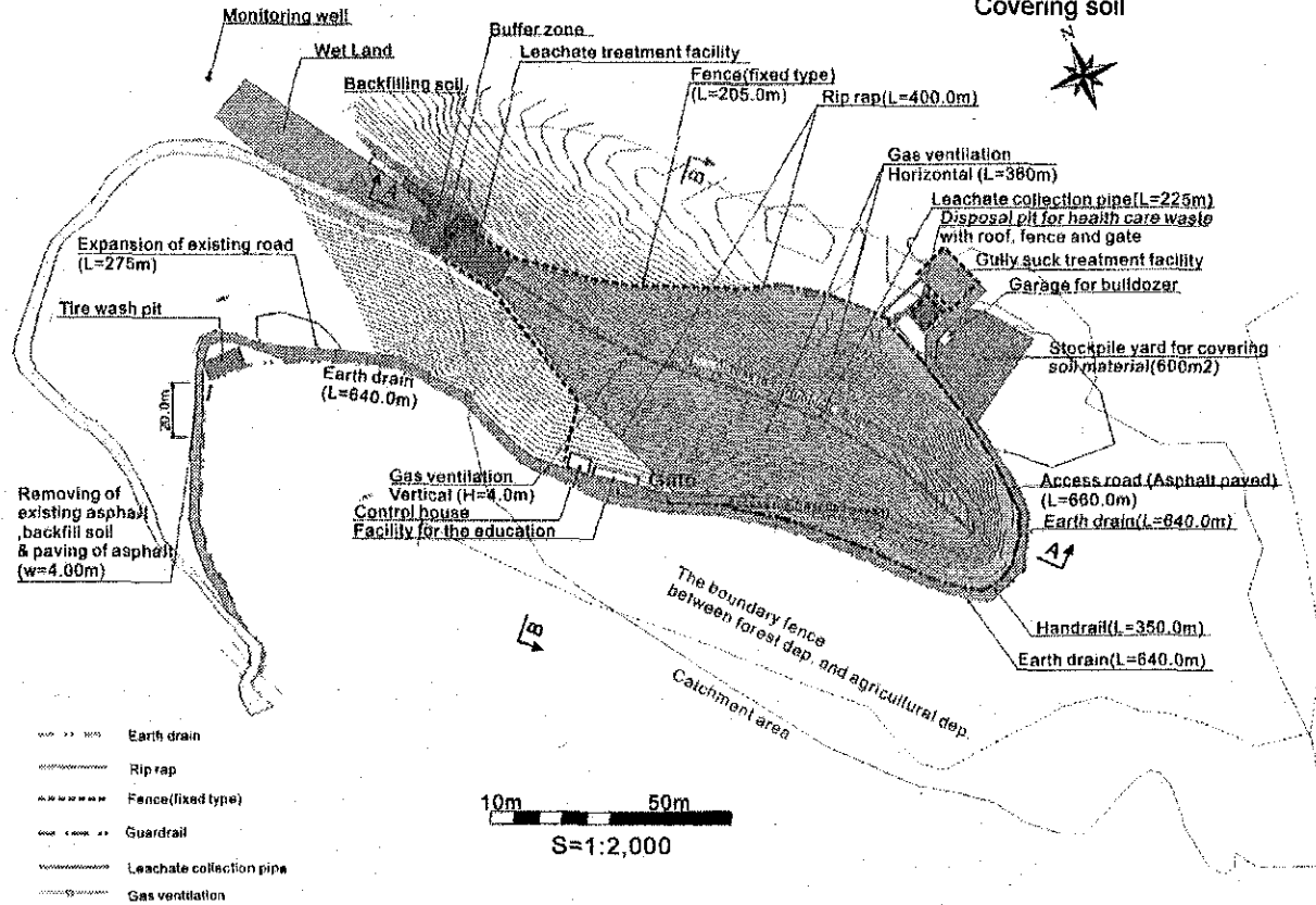
Figure H.2-3: Layout Plan of Improved Landfill Site
