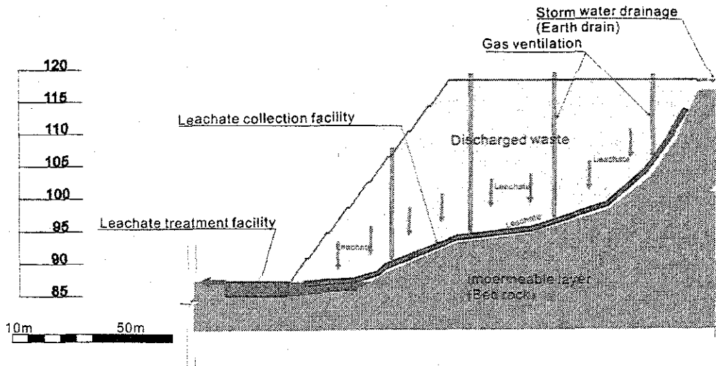
Figure H.2-4: Leachate Treatment Facility for Blocking Leachate
