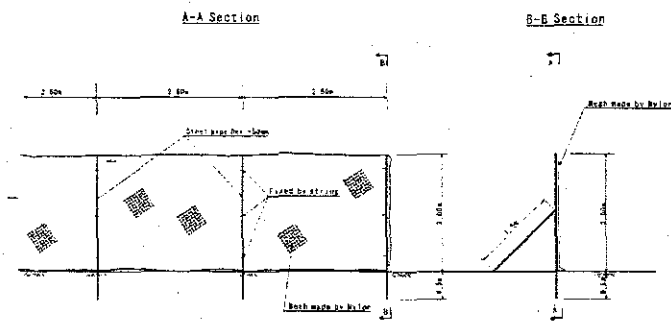
Figure H.2-7: Fence (movable type)
