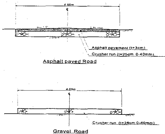
Figure H.2-18: Typical Cross Section of Access Road
