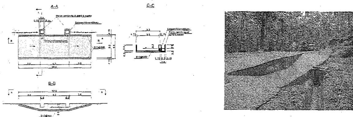
Figure H.2-11: Tire Wash Pit
