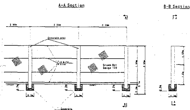
Figure H.2-16: Fence (fixed type)
