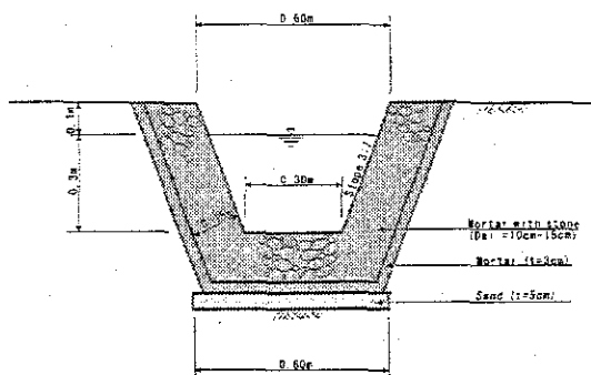
Figure H.2-8: Riprap Lined Storm water Drain
