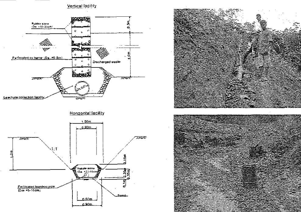
Figure H.2-9: Gas Venting Facility
