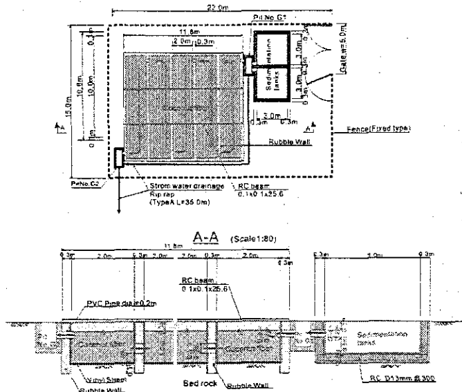
Figure H.2-12: Gully Suck Facility
