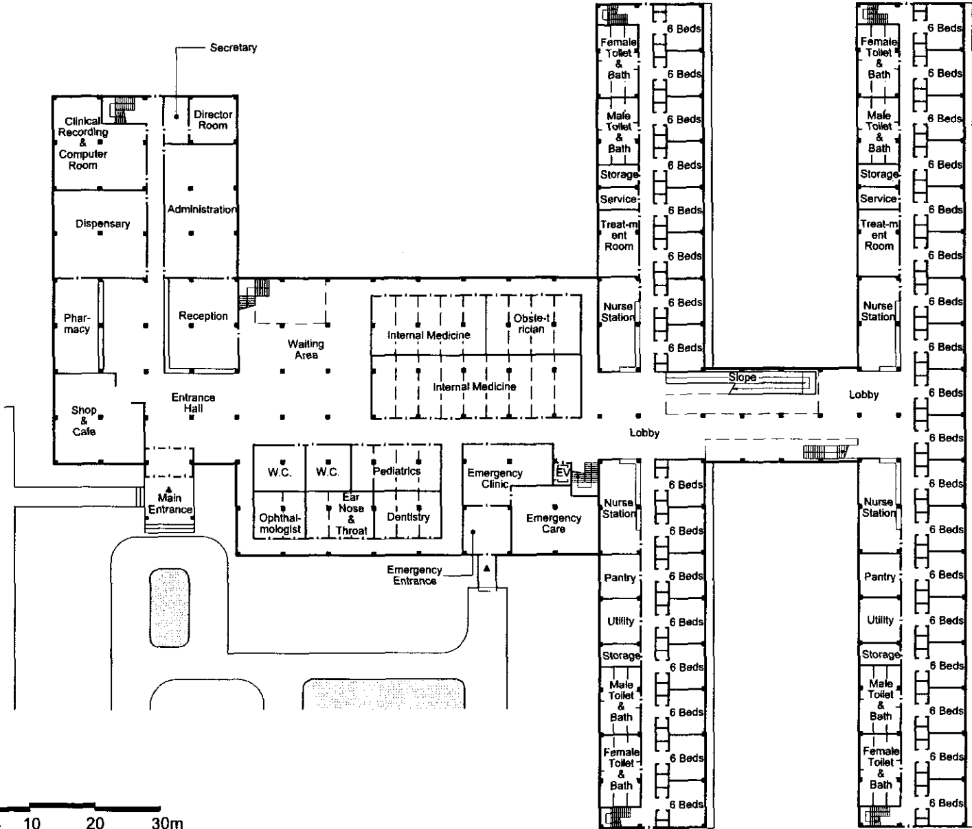
Appendix Figure 16.1.2 Recommended Oblast General Hospital Construction Plan
