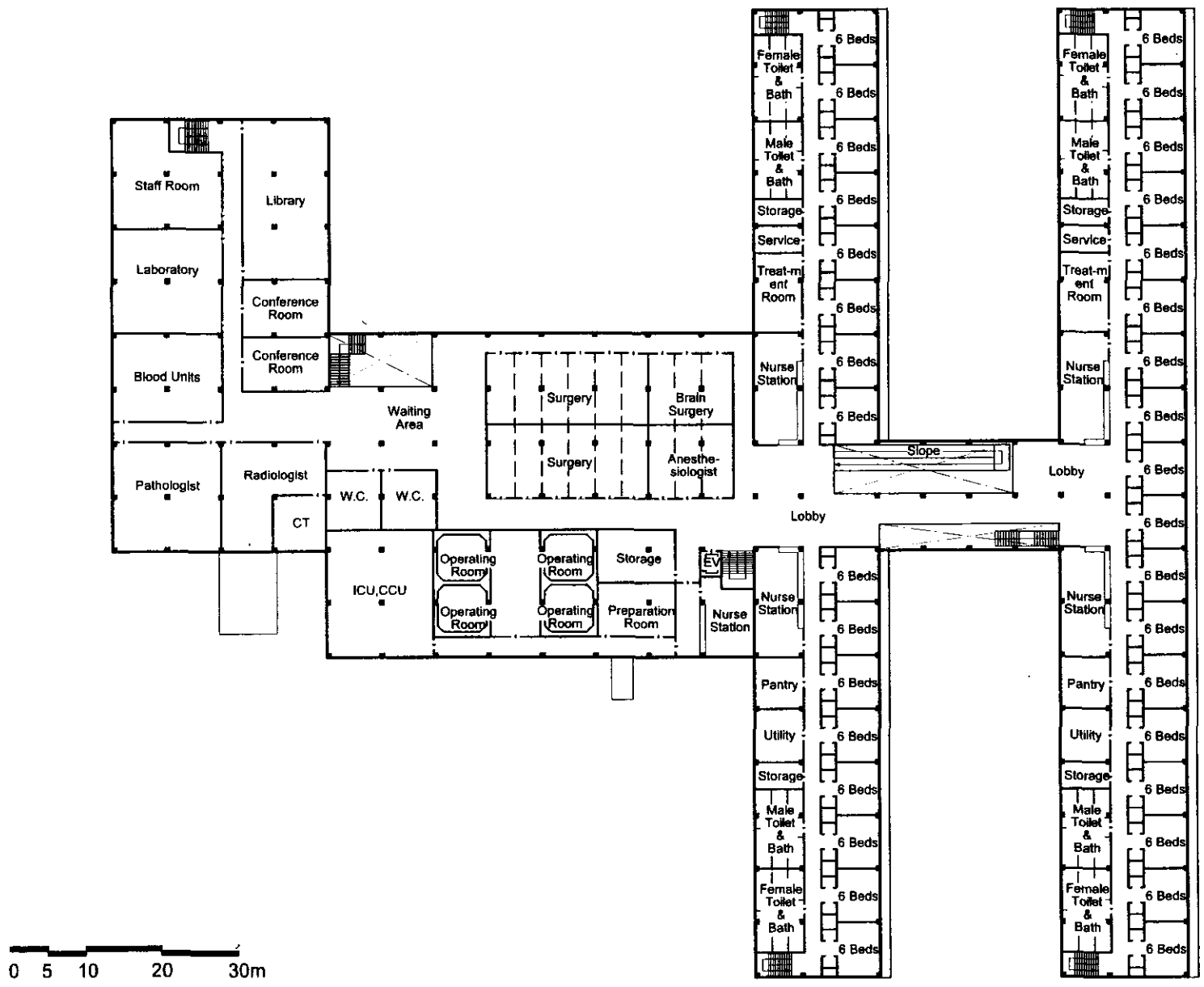
Appendix Figure 16.1.3 Recommended Oblast General Hospital Construction Plan
