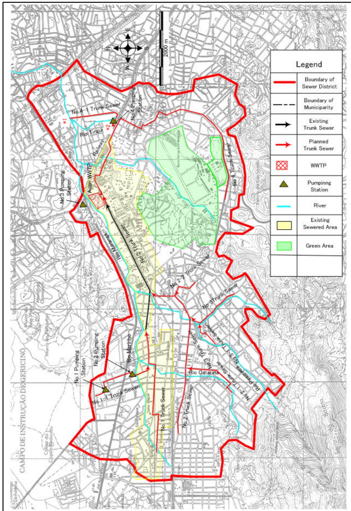
Figure 7.6 Layout Plan of Acarí Sewer District
