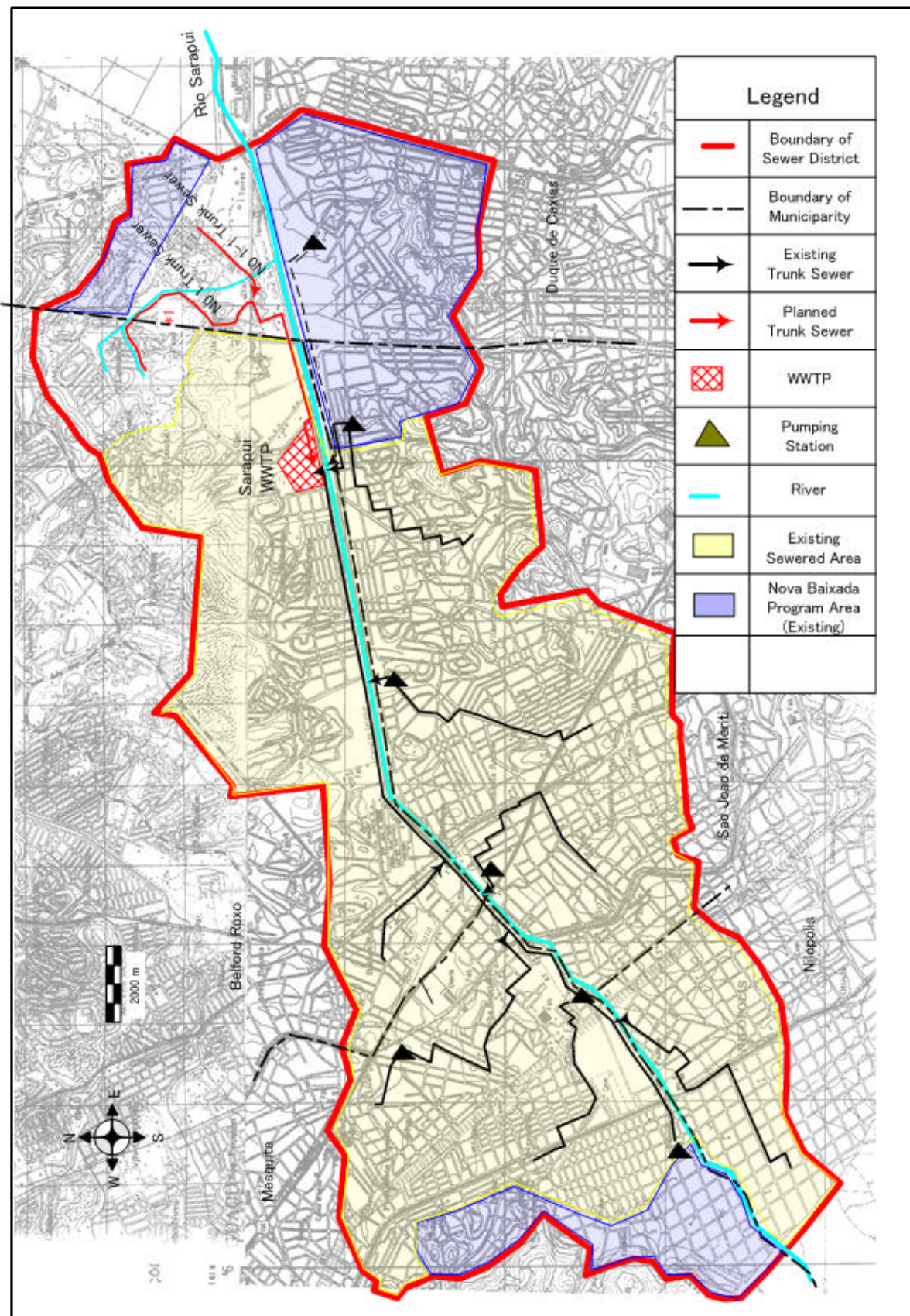
Figure 7.8 Layout Plan of Sarapuí Sewer District
