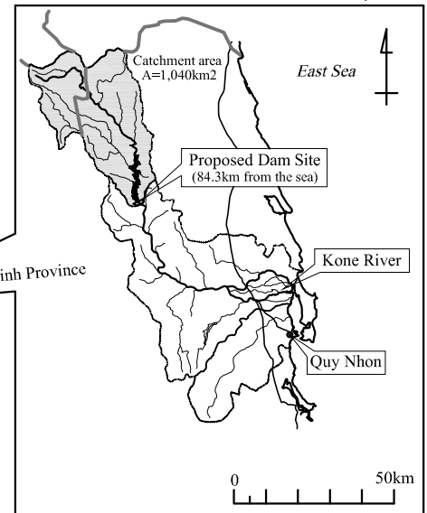
Figure 9.1 Location Map of Dinh Binh Damsite
