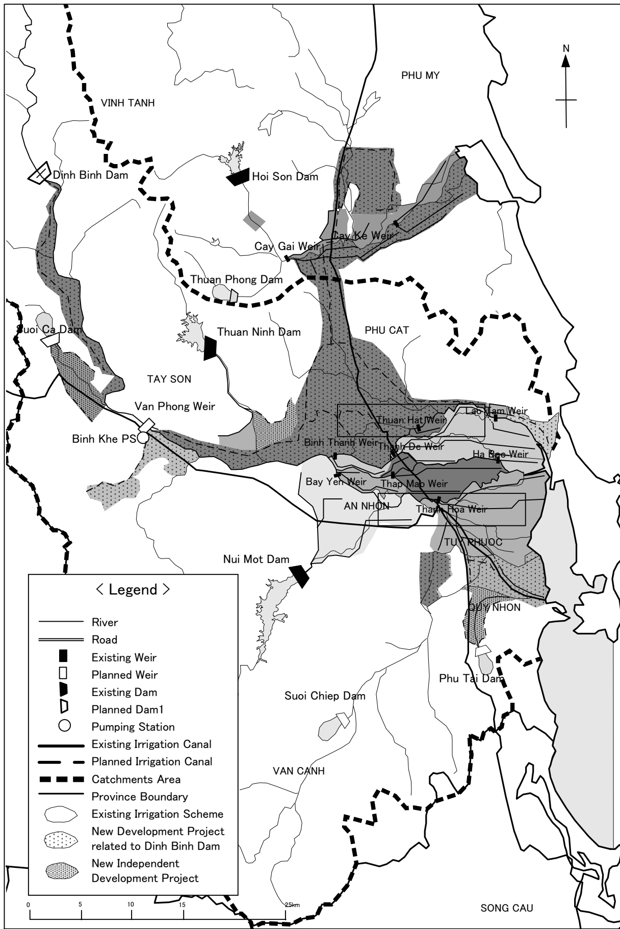
Figure 8.5 General Layout of Irrigation Development Plan
