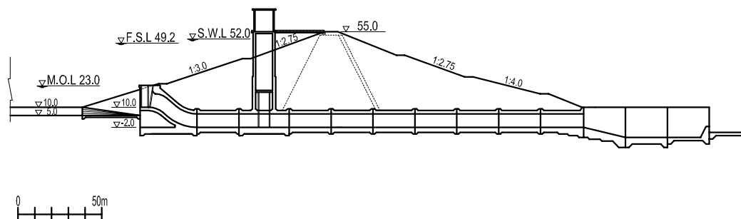
Section C - C
