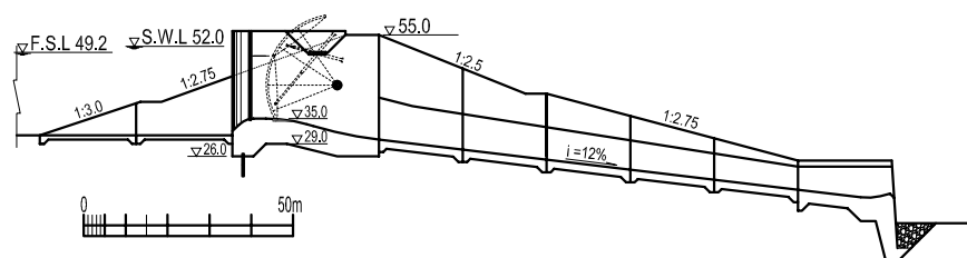
Figure 9.27 Ta Trach Multi-purpose Reservoir
