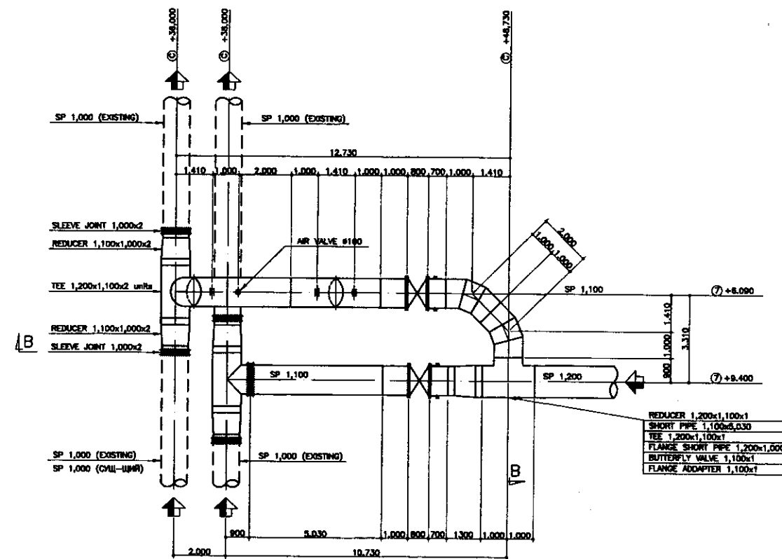
DETAIL (C) / ДЕТАЛЬ (C) SCALE 1:100
