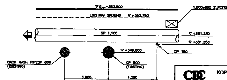
SECTION D-D/PA3PE3 D-D SCALE 1:100
