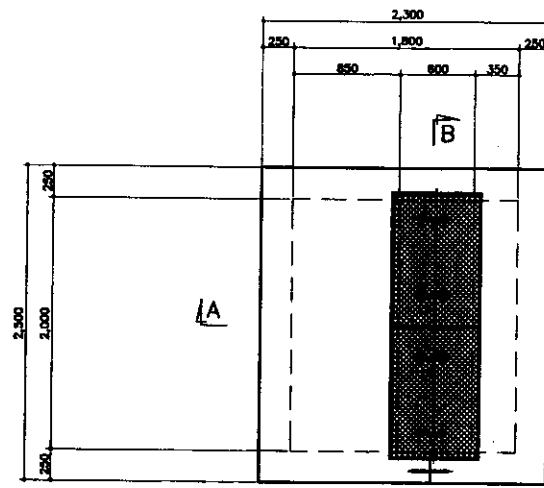
TOP PLAN SCALE 1:30
