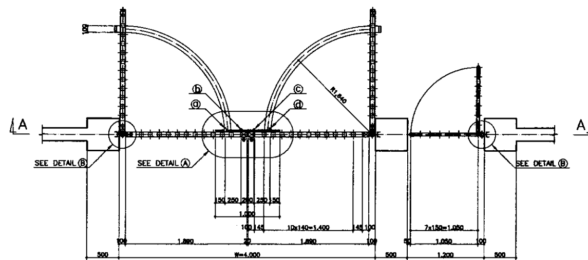
PLAN SCALE 1:30
