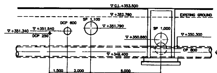
SECTION C-C/PA3PE3 C-C SCALE 1:100
