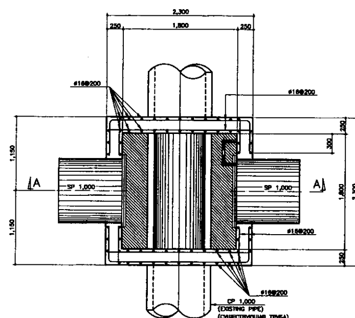
BOTTOM PLAN SCALE 1:30
