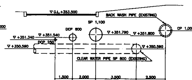
SECTION B-B/PA3PE3 B-B SCALE 1:100
