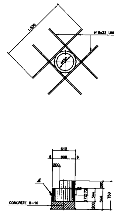
DETAIL ① SCALE 1:30
