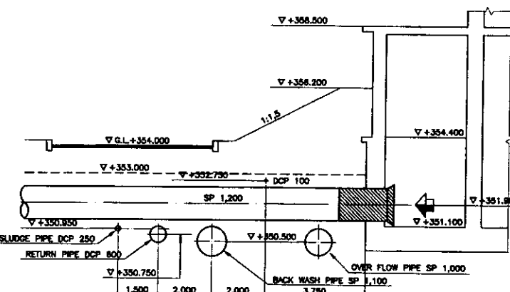
SECTION E-E/PA3PE3 E-E SCALE 1:100
