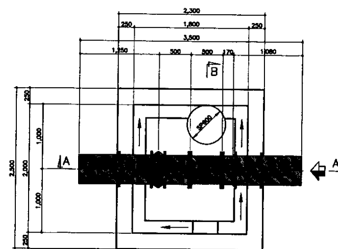
BOTTOM PLAN SCALE 1:30
