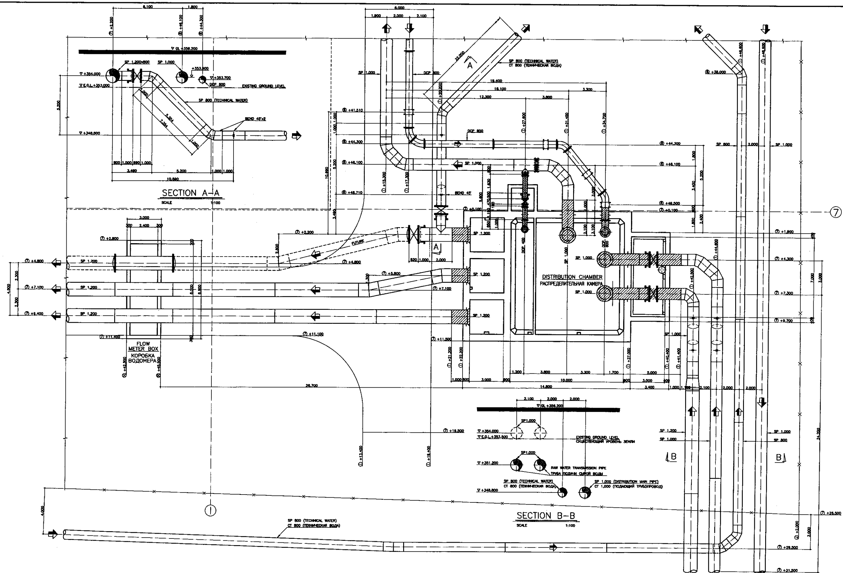
DETAIL (A) SCALE 1:100
