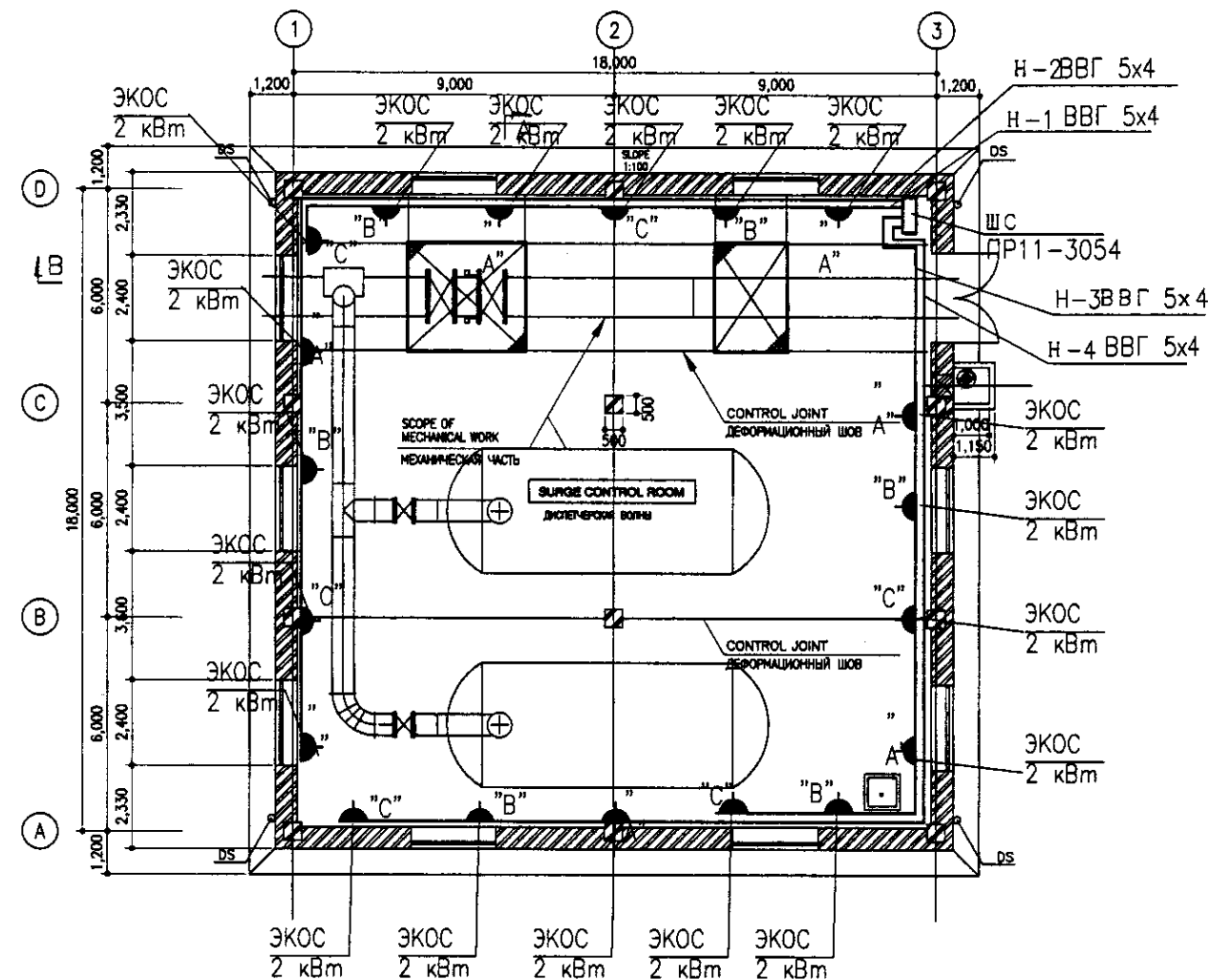
FLOOR PLAN
