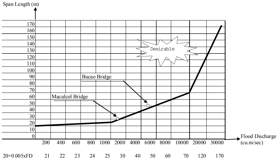
Figure 1 Span Length
