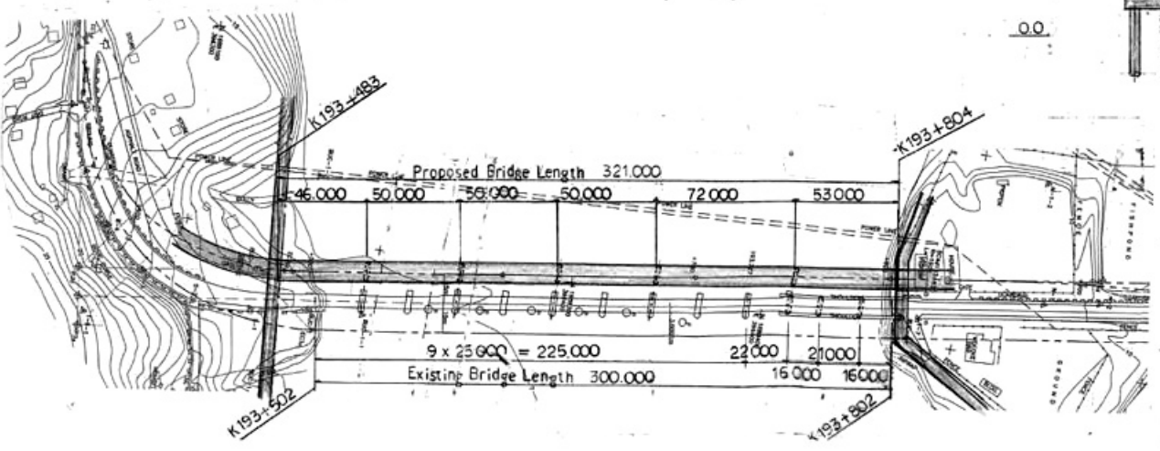
Figure 1.3.8 General View of the Bucaco Bridge for Reconstruction
