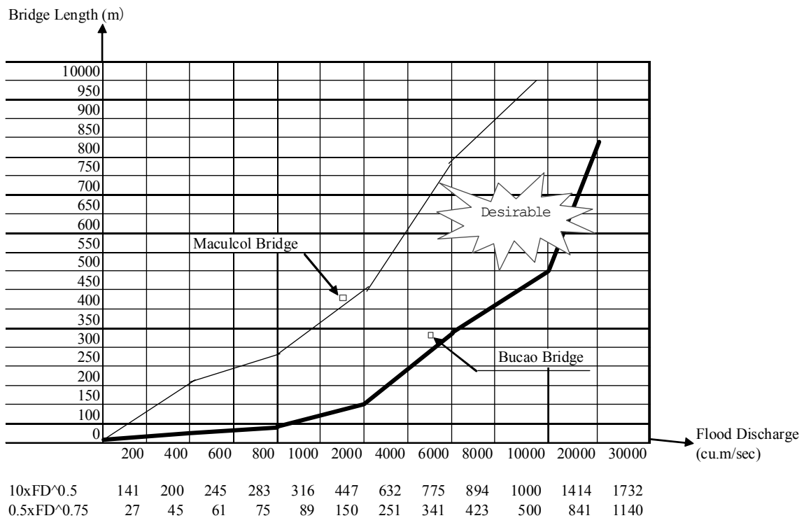
Figure 2 Bridge Length
