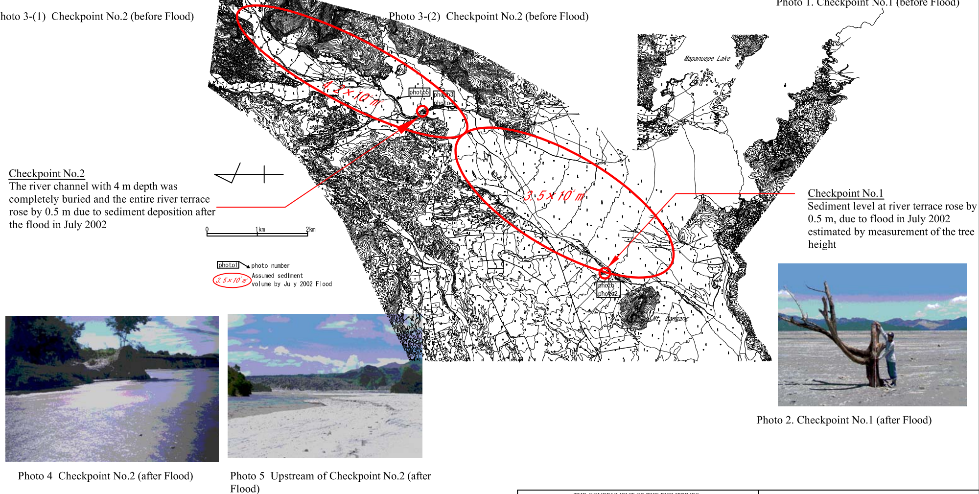
Figure 6.2.3 Investigation Results of Sediment Delivery in 2002 in the Marella River
