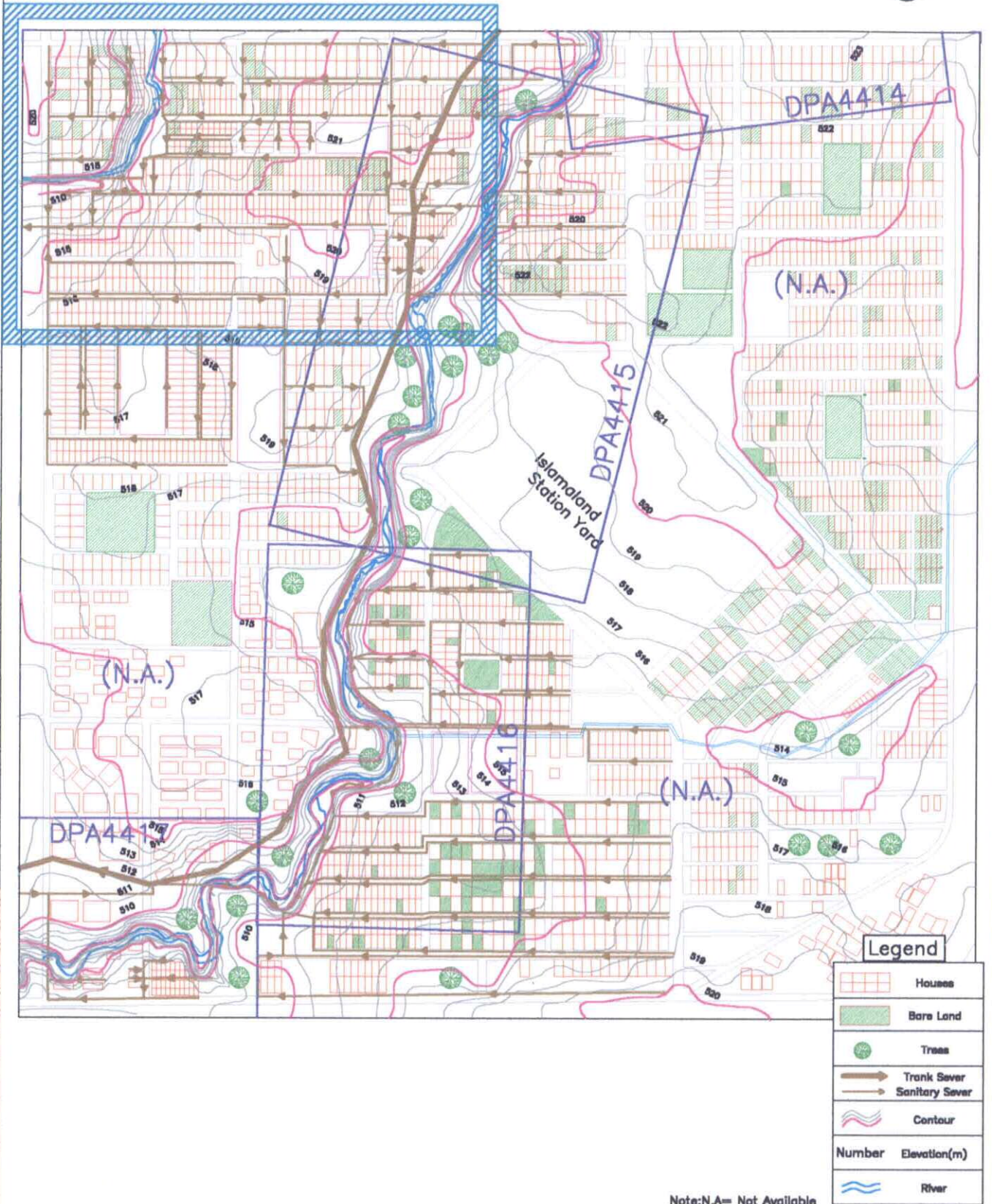
Fig. F.4 Sewerage System in I-8, Islamabad
