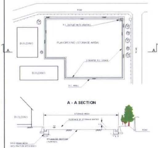
PLAN OF STORAGE IN PUBLIC SPACE
