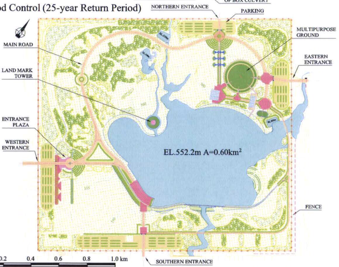
Fig. C.5 Plan of Community Pond
