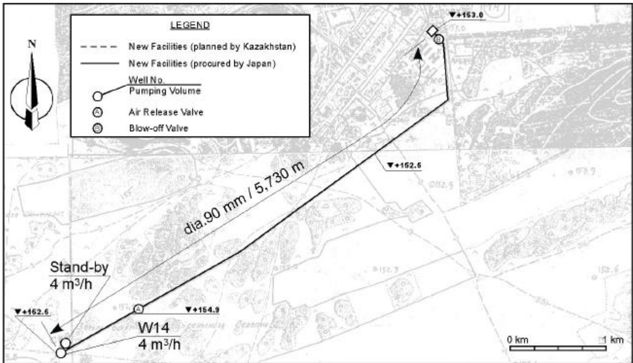
Water Transmission Pipeline (No.14 Kirovka)
