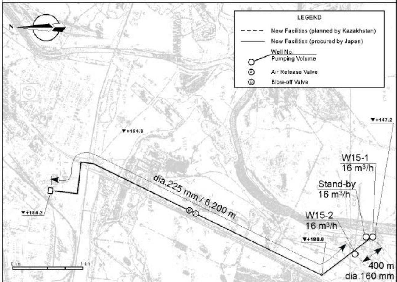
Water Transmission Pipeline (No.15 Novoishimsky)
