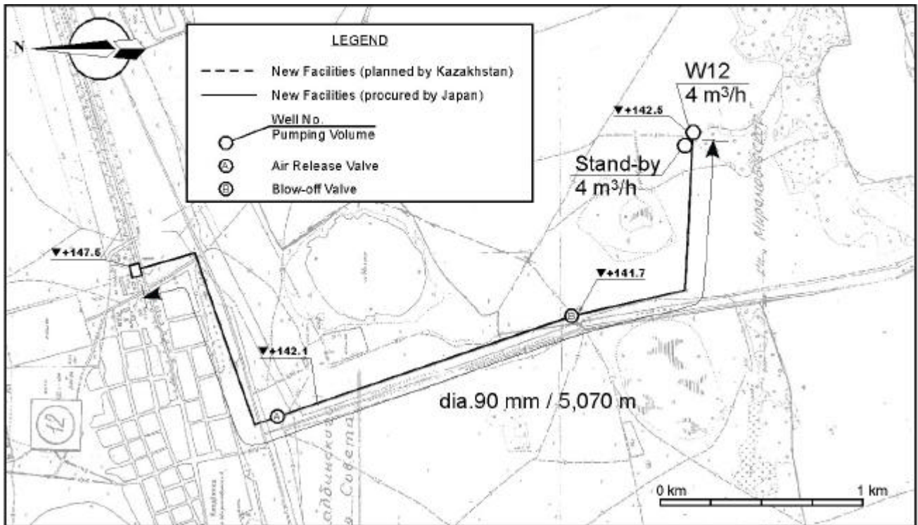
Water Transmission Pipeline (No.12 Kladbinka)
