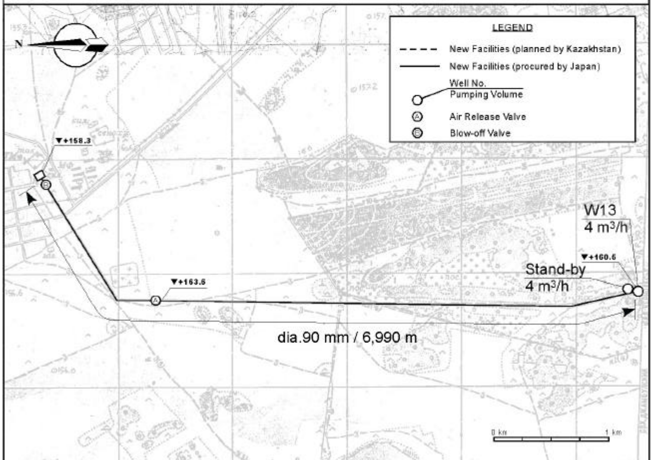
Water Transmission Pipeline (No.13 Maibalyk)
