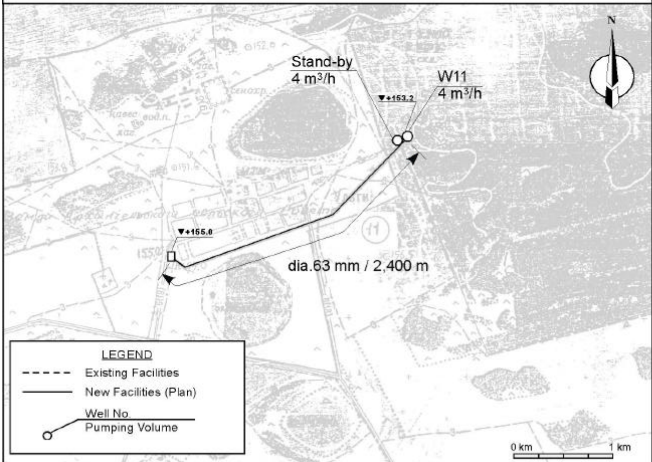
Water Transmission Pipeline (No.11 Ulgy)
