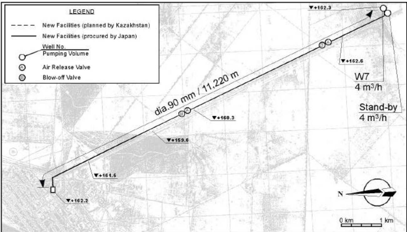
Water Transmission Pipeline (No.7 Korneevka)
