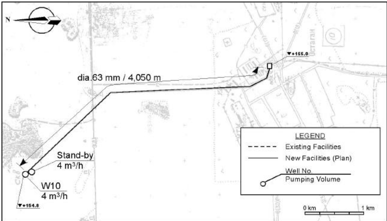
Water Transmission Pipeline (No.10 Ostagan)
