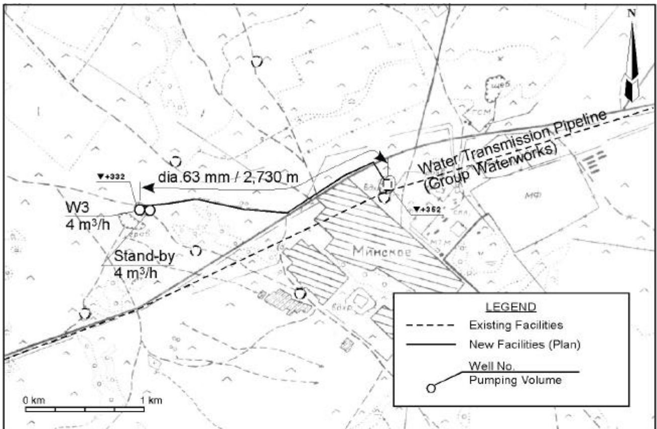
Water Transmission Pipeline (No.3 Minskoye)
