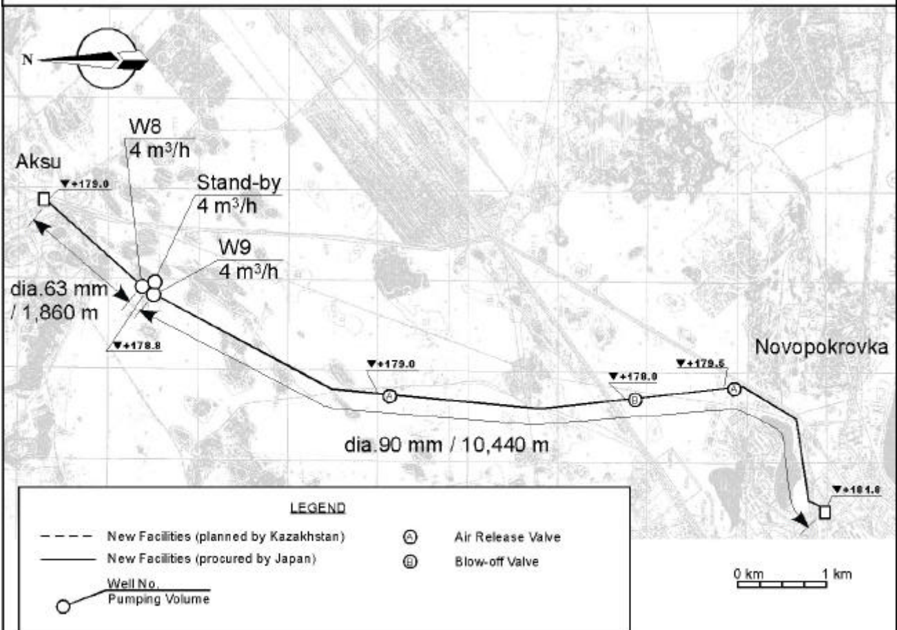
Water Transmission Pipeline (No.8 Aksu, No.9 Novopokrovka)
