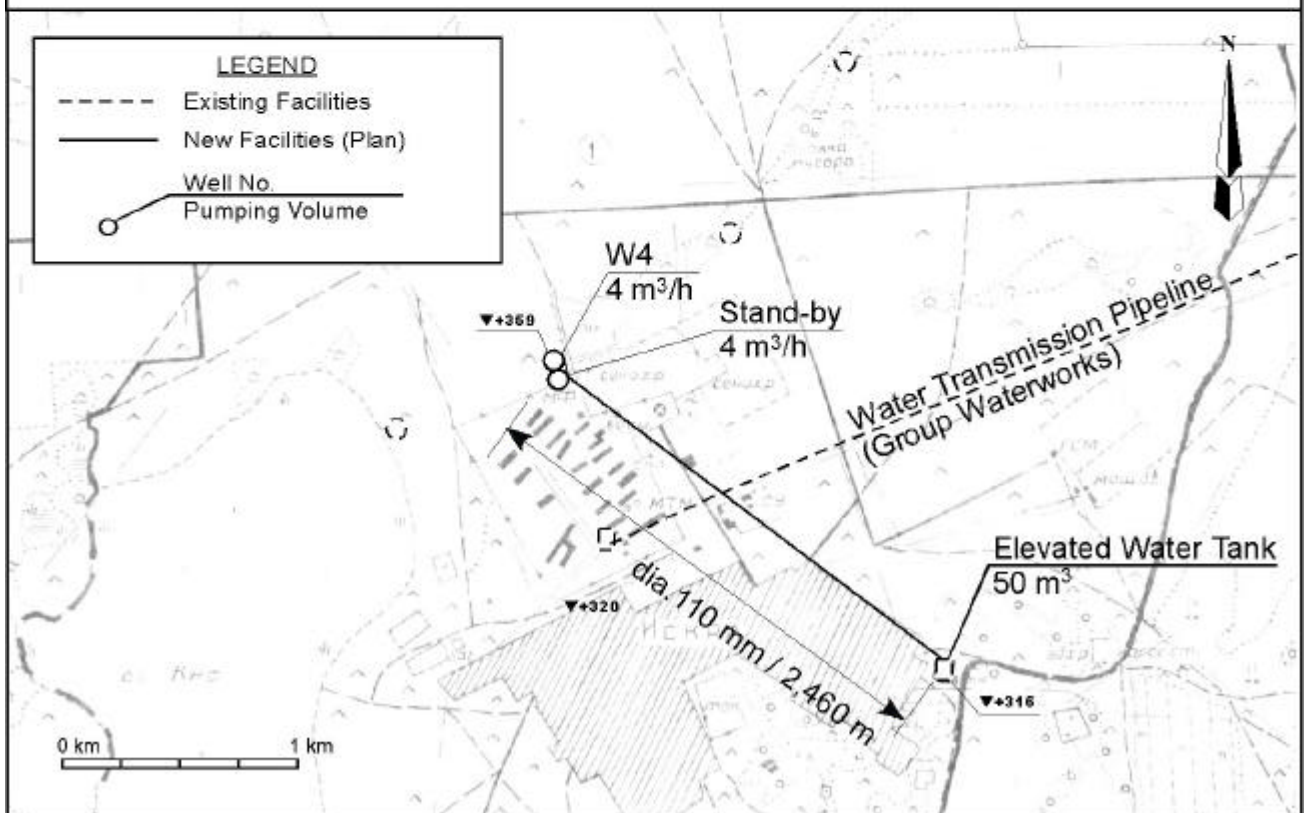
Water Transmission Pipeline (No.4 Iskra)
