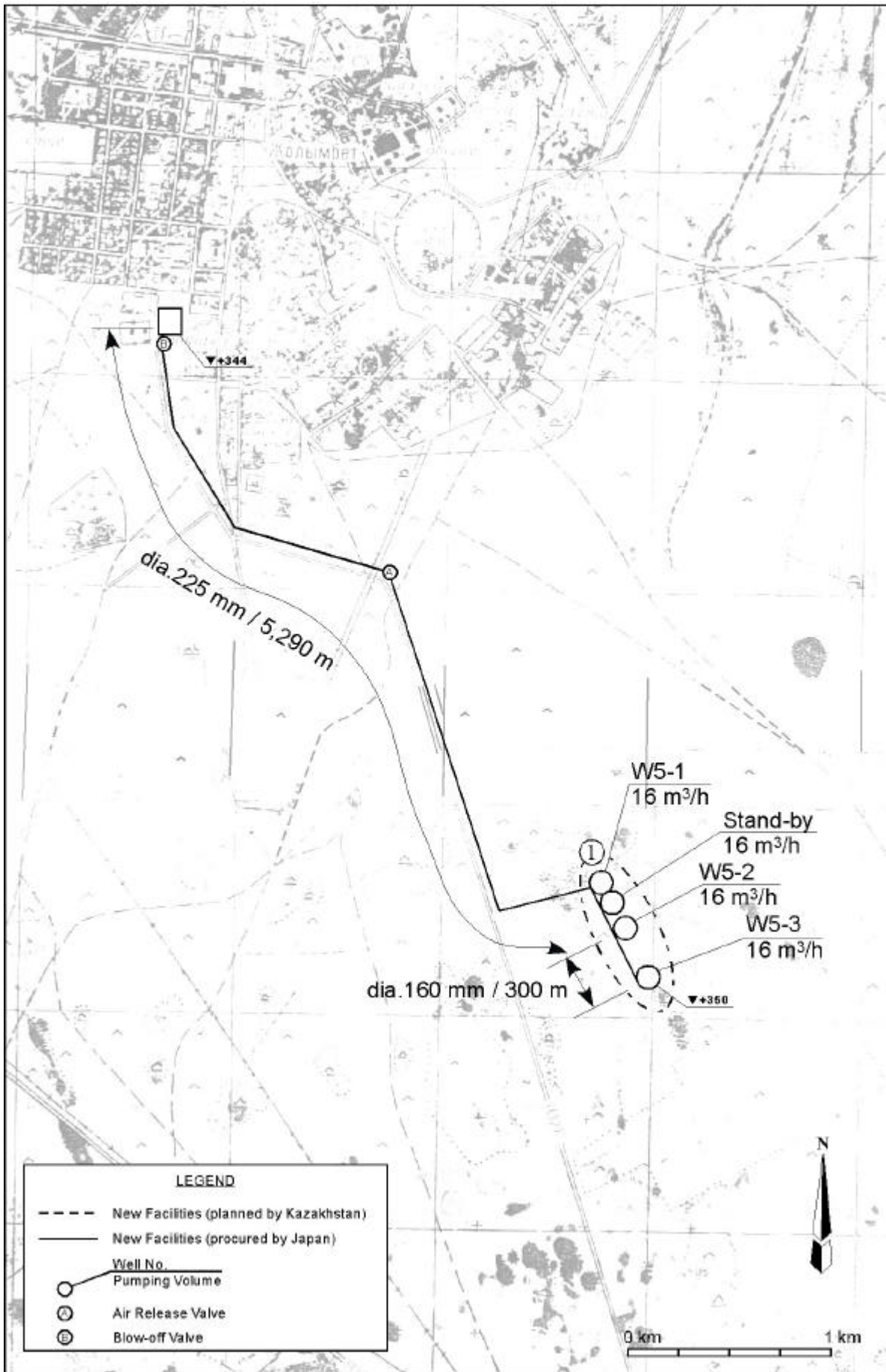
Water Transmission Pipeline (No.5 Zholymbet)
