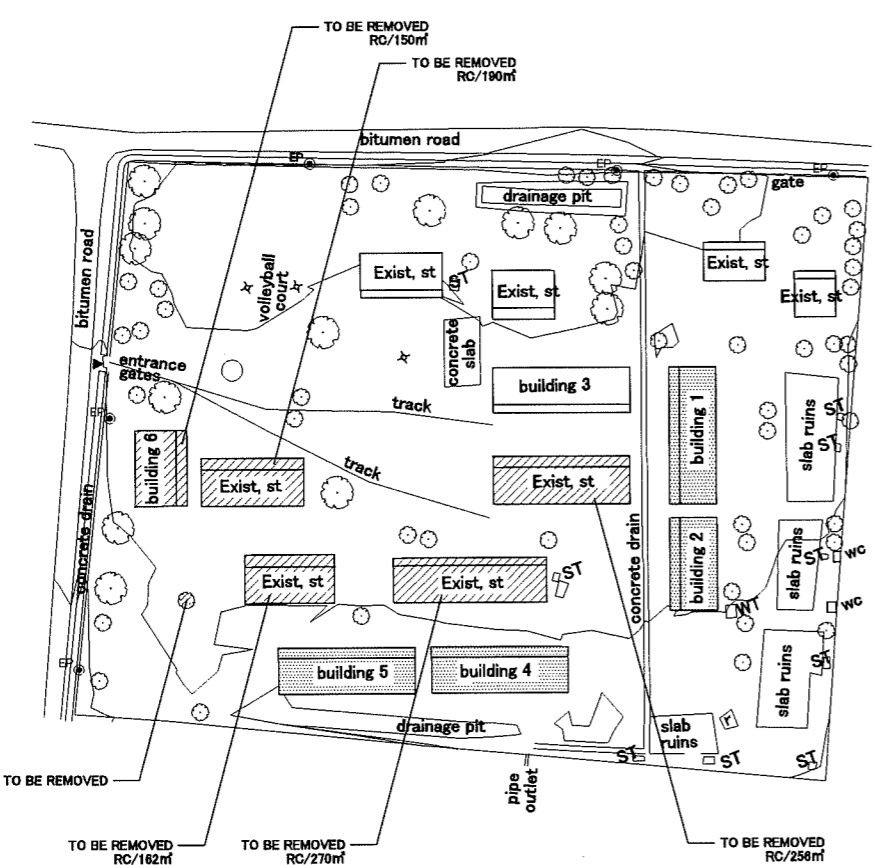
EXISTING SITE DEVELOPMENT PLAN SCALE 1:1500M
