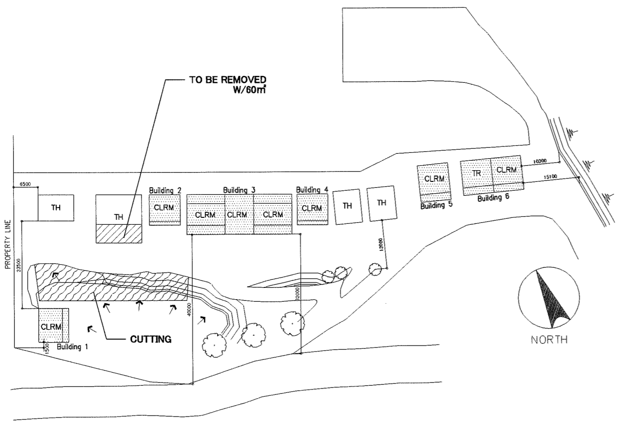
EXISTING SITE DEVELOPMENT PLAN SCALE 1:1000M
